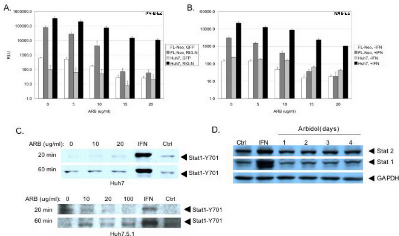
Figure 4 ARB does not induce IFN antiviral responses. A, ARB does not induce RIG-I dependent signaling. FL-Neo replicon and Huh7 cells were co-transfected with IFNB-luciferase and GFP or IFNB-luciferase and constitively active RIG-N expressing plasmids for 3 hours. Transfection mixtures were then removed and cells were incubated with medium containing the indicated concentrations of ARB. Luciferase activity was measured 24 hours later. B, ARB does not induce ISRE transcription. FL-Neo and Huh7 cells were transfected with ISRE-luciferase reporter plasmids for 3 hours. Transfection mixtures were then removed and cells were incubated with medium containing the indicated concentrations of ARB for 20 hours. Cells were then treated or not treated with 100 U/ml of IFN- \alpha (Roferon) for 4 hours before luciferase activity was measured. C, ARB does not induce Stat1 phosphorylation on the conserved tyrosine amino acid at position 701. Huh7 or Huh7.5.1 cells were treated with the indicated amounts of ARB and whole cell protein extracts were harvested 20 and 60 minutes later. Cells were also treated with 500 units per milliliter of IFN- \alpha , or as a negative control for possible solvent effects, an equivalent volume of ethanol (Ctrl). The position of Stat1-Y01 is indicated with arrows. D, ARB does not induce IFN stimulated gene expression. FL-Neo cells were treated with 6 \mu g/ml ARB for 1 to 4 days, or treated with 100 U/ml IFN- \alpha for 24 hours. Whole cell protein extracts were probed for Stat1, Stat2, and GAPDH protein levels.
