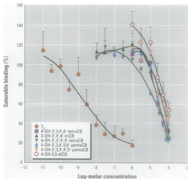
Figure 5. Competitive binding of hydroxylated polychlorinated biphenyls to recombinant human thyroid receptor β. Assay conditions are as described in Figure 4. n = 3 experiments performed in duplicate. Abbreviations: T 3 , 3,3',5-triiodothyronine; CB, chlorinated biphenyl.
