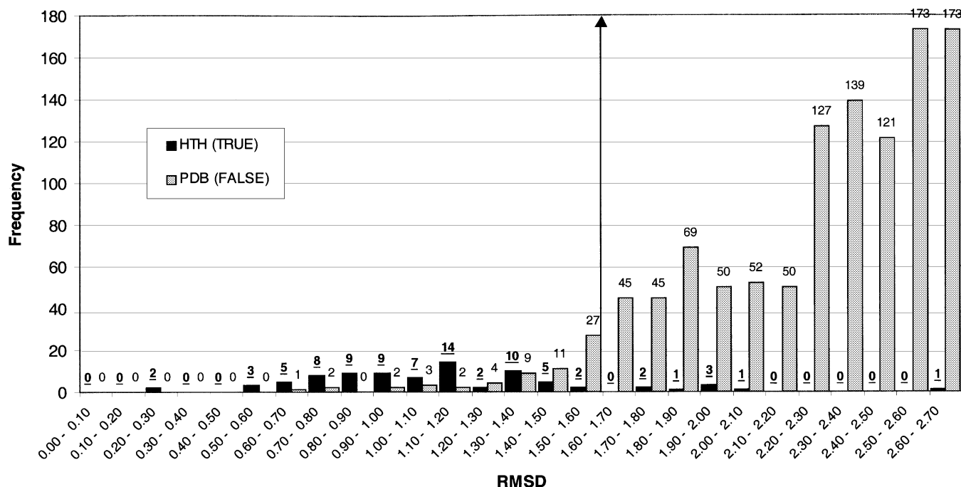
Figure 6. Frequency histogram showing the distribution of rmsd values resulting from a scan of seven HTH templates against 86 HTH proteins ( HTH X HTH ) and 8264 PDB proteins (excluding known HTH proteins) ( HTH X FALSE ). The HTH X HTH distribution is shown in black and the HTH X FALSE distribution is shown in grey. The maximum rmsd shown is 2.7 Å. A threshold value is indicated at 1.6 Å, below which a protein is predicted to contain a DNA-binding HTH motif.
