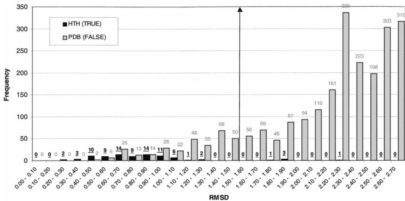
Figure 4. Frequency histogram showing the distribution of rmsd values resulting from a scan of seven HTH templates against 84 HTH proteins ( HTH X HTH ) and 8266 PDB proteins (excluding known HTH proteins) ( HTH X FALSE ). The HTH X HTH distribution is shown in black and the HTH X FALSE distribution is shown in grey. The maximum rmsd shown is 2.7 Å. A threshold value is indicated at 1.6 Å, below which a protein is predicted to contain a DNA-binding HTH motif.
