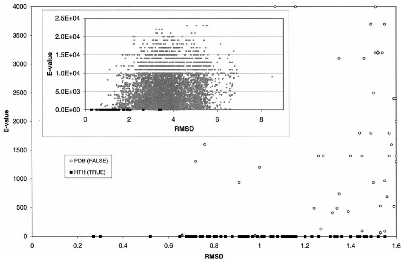
Figure 7. Scatter plot of E values derived from HMM scans of protein sequence against rmsd values from 3D extended motif scans of protein structure. The inset graph shows the distribution of rmsd values up to a maximum of 8.5 Å and E values to a maximum of 2.5E + 04 with values rounded to two significant figures as recorded in the results from SAM-T99. The main graphs show the distribution with rmsd values to a maximum of 1.6 Å and E values to a maximum of 4000. The data points for the 86 known HTH motifs (TRUE) are shown in filled black squares, those for the remaining PDB structures not known to contain DNA binding HTH motifs (FALSE) are shown as open grey circles. The filled grey diamonds indicate the two structures (1fy7A and 1mgtA) both predicted to include DNA-binding HTH motifs. These data are derived from the third scan of the PDB with seven non-homologous extended HTH motifs.
