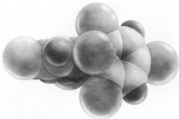
FIGURE 3. Model of 2,2',4,4',6,6'-hexachlorobiphenyl (congener number 155) illustrating steric hindrance to rotation of the rings imposed by substitution of the maximum possible number of chlorine atoms (four) at the ortho positions of the molecule. Rings are shown rotated at the angle of preferred orientation, 87.3°.
