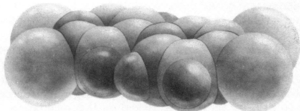
FIGURE 4. Model of 3,3',4,4'-tetrachlorobiphenyl (congener number 77) shown in coplanar conformation. Large spheres at ends of the molecule are the four chlorine atoms.
