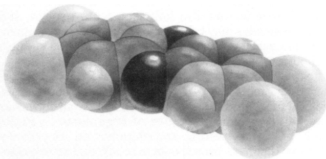
FIGURE 2. Molecular model of 2,3,7,8-tetrachlorodibenzo- p -dioxin. Dark spheres are oxygen atoms. The four large light spheres at the ends of the molecule are chlorine atoms.
