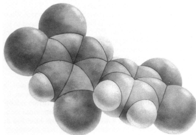
FIGURE 5. Model of 2,3',4,4',5-pentachlorobiphenyl (congener number 118), a mono- ortho chlorine substituted PCB having mixed-type MFO-inducing properties (see text). Rings are shown rotated at 46.6°.
