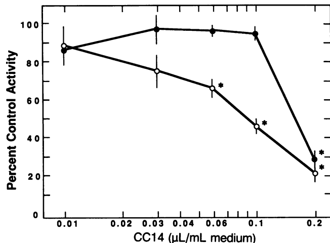
FIGURE 3. ER and mitochondrial calcium sequestration in material isolated from hepatocytes exposed to \text{CCl}_4 . Hepatocyte cultures were exposed to \text{CCl}_4 (0.01 to 0.2 \mu\text{L}/\text{mL} or vehicle for 5 min). Cells were then homogenized and promptly assayed under conditions optimized for ^{45}\text{Ca} sequestration by ER (○) or mitochondria (●). Results are expressed as mean \pm SEM. In control cultures, mitochondrial calcium sequestration averaged 58.4 \pm 9.7 nmole calcium/mg protein/10 min and ER calcium pump averaged 94.1 \pm 9.9 nmole calcium/mg protein/30 min. Differences are significant where indicated ( p \leq 0.05 ) by ANOVA (17).
