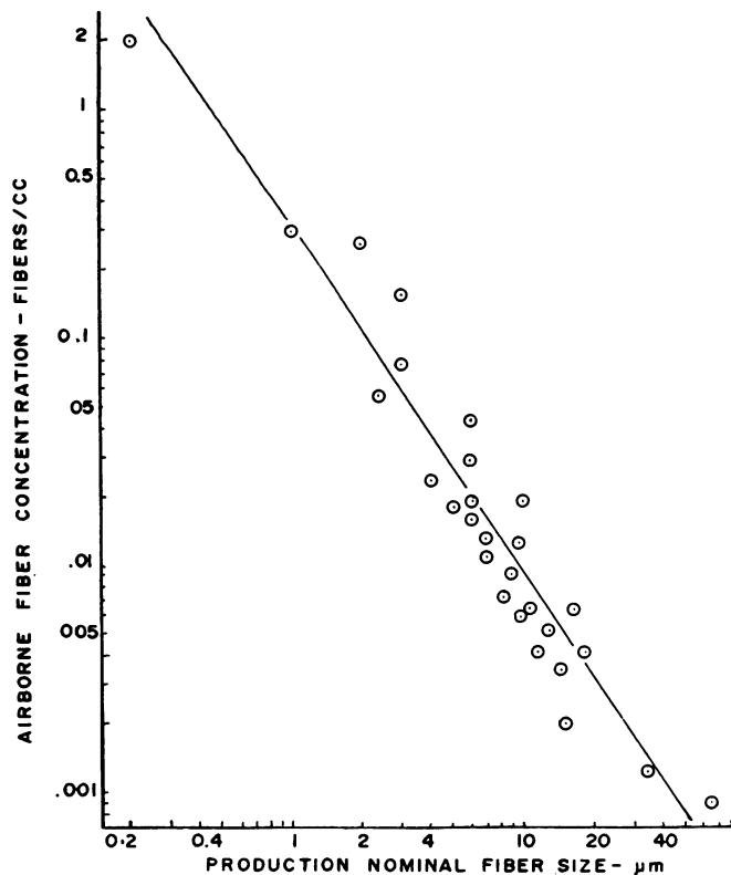
FIGURE 2. Relationship between measured average exposures, expressed as fibers per cubic centimeter and nominal diameter of fiber manufactured. Fibers per cubic centimeter determined by phase contrast microscopy.
