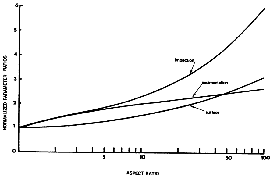
FIGURE 1. The relationship between normalized ratios of aerodynamic sedimentation and impaction diameters to the fiber diameter of the fiber surface to spherical surface of equal volume as a function of aspect ratio.
