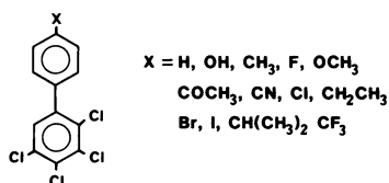
FIGURE 7. Structure of the model ligands.
