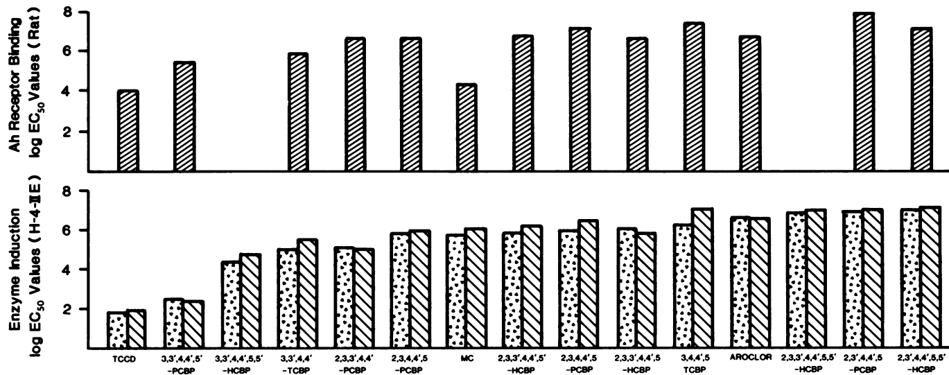
FIGURE 2. AHH/EROD induction potencies (bottom) and cytosolic receptor protein binding affinities of coplanar and mono- ortho coplanar PCB isomers and congeners. □ EROD; ▨ AHH; ▩ Ah receptor binding.
