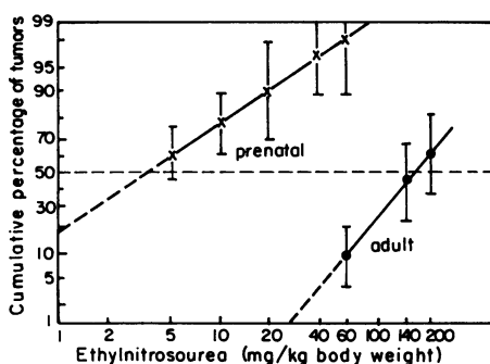
FIGURE 8. Dose-response relationships for the prenatal induction of malignant tumors of the nervous system compared with that in adult rats. Ethylnitrosourea was administered as a single dose. Adapted from Druckrey et al. (28).
