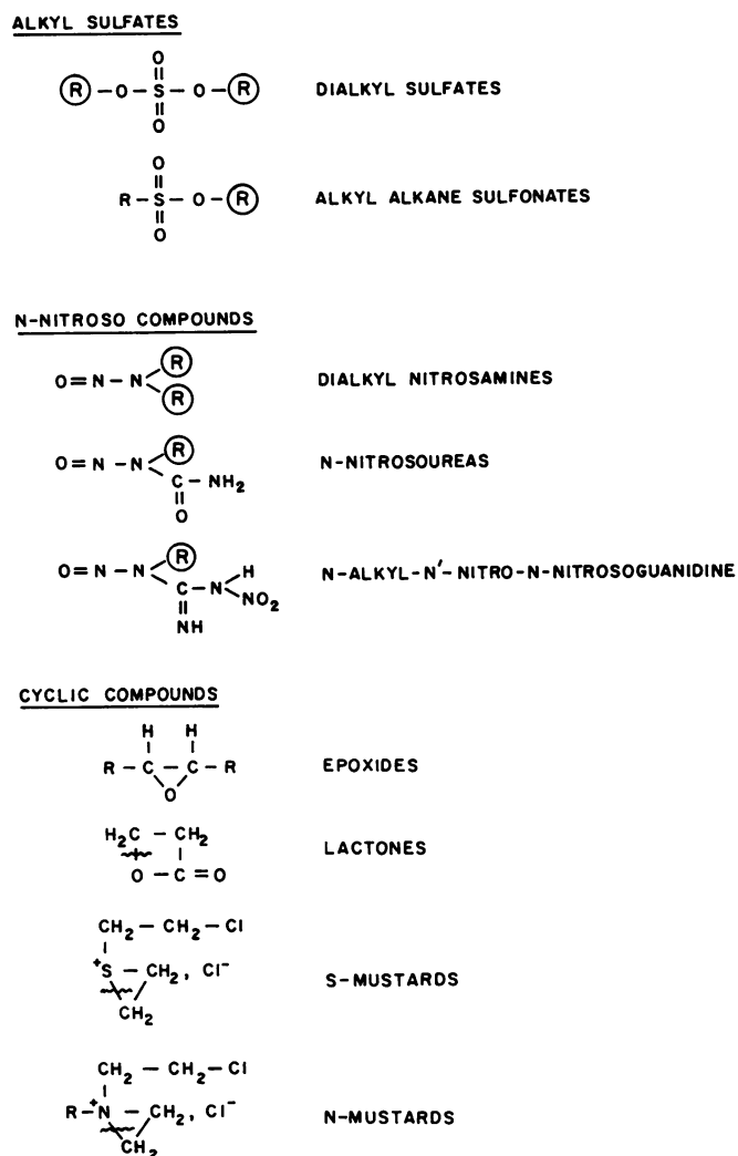
FIGURE 1. Structural formulas of simple alkylating agents. All are direct acting except dialkyl nitrosamines, which must be metabolically activated. The cyclic compounds owe their alkylating ability to reactive, unstable ring structures.
