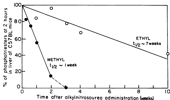
FIGURE 7. Loss of methyl and ethyl phosphotriesters from liver DNA of C57BL mice given a single injection of methylnitrosourea or ethylnitrosourea. Phosphotriesters were determined from the extent of degradation induced in isolated DNA by alkali. Data from Shooter and Slade (34).
