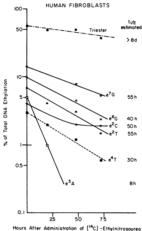
FIGURE 4. Amounts of ^{14}\text{C} ethyl products from ethyl nitrosourea-treated mammalian cells, prelabeled with ^3\text{H} . The initial proportion of total ethylation is shown on the log scale. All values have been corrected for cell division. The estimated t_{1/2} of derivatives is shown in the figure. Adapted from Bodell et al. (14).
