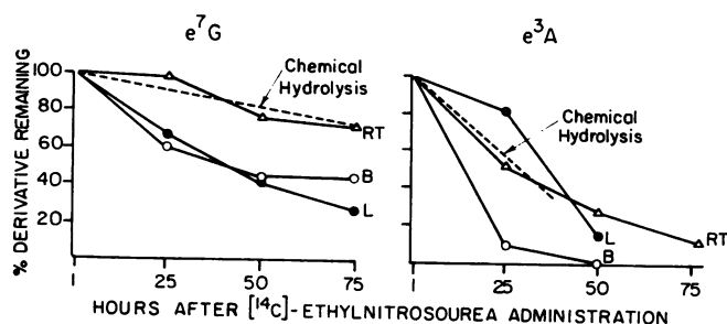
FIGURE 6. Stability of e^7\text{G} (7-ethyl G) and e^3\text{A} (3-ethyl A) in DNAs in ethylnitrosourea-treated 10-day-old BD IX rats (30), as compared to the chemical stability in vitro ( \Delta ): (---) rate of chemical hydrolysis at pH 7, 37°C; (○) brain; (●) liver; ( \Delta ) other tissues, pooled.
