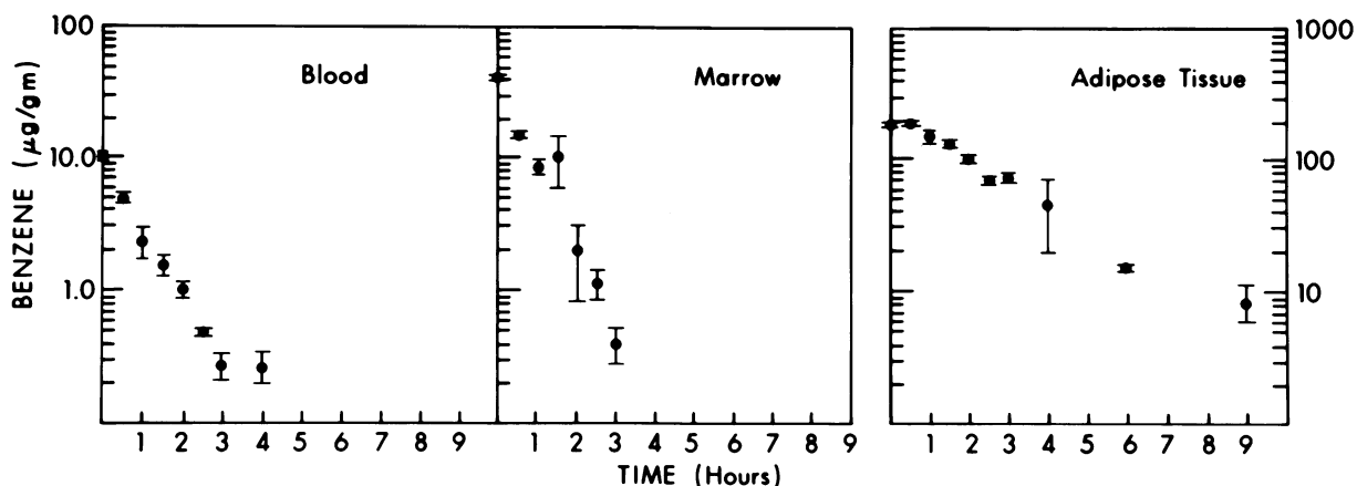
FIGURE 3. Disappearance of benzene from blood, bone marrow, and adipose tissue following 6 hr exposure to 500 ppm benzene in air.
