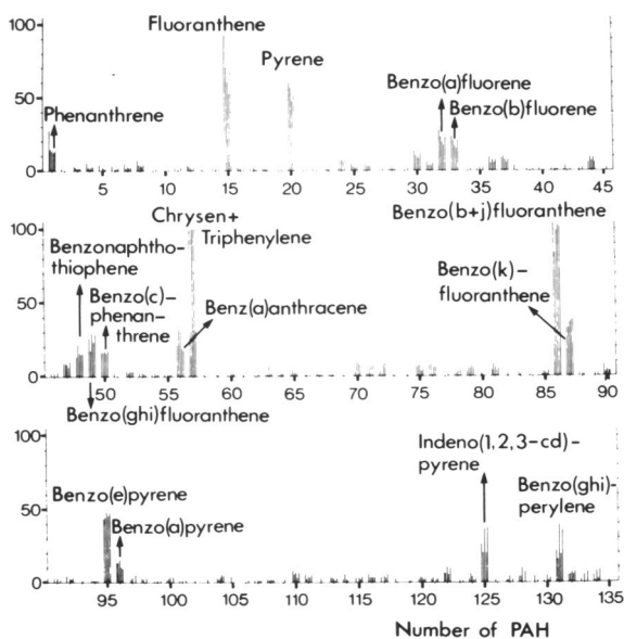
FIGURE 11. Relative amounts of 135 PAHs (chrysen = 100) isolated from extracts of suspended particulate matter collected in five cities in West Germany. The five columns in each group correspond to Bremen, Duisburg, Frankfurt, Karlsruhe and Munich (30).
