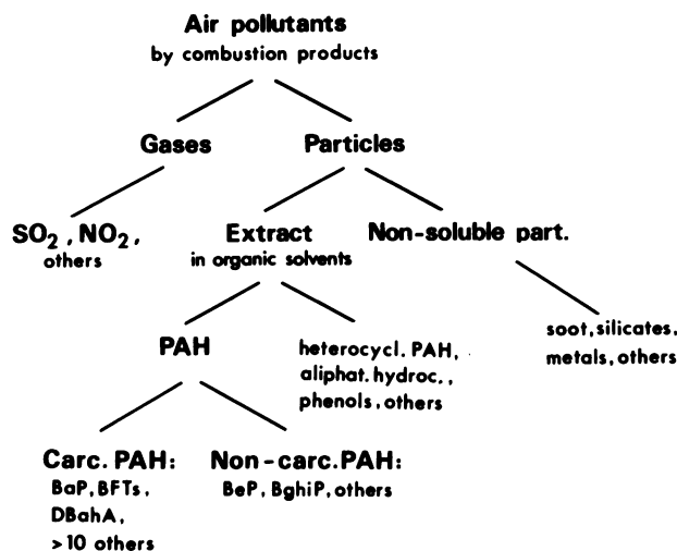
FIGURE 1. Rough scheme of the fractionation of air pollutants from combustion emissions for the examination of the carcinogenicity of specific groups of compounds; BaP = benzo(a)pyrene; BFTs = benzo(b)fluoranthene; DBahA = dibenz(a,h)anthracene; BeP = benzo(e)pyrene; BghiP = benzo(ghi)perylene.
