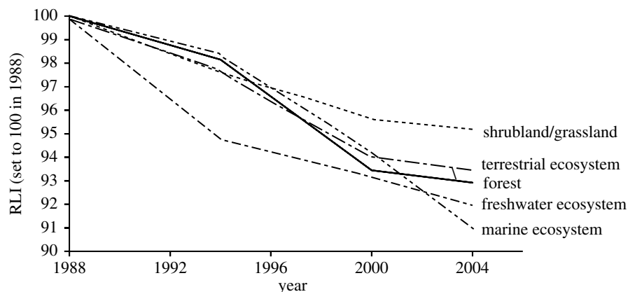
Figure 5. Red List Indices for birds for 1988–2004 in the marine, freshwater and terrestrial ecosystems, and for birds in forest and shrubland/grassland habitats. Sample sizes: marine = 12 genuine status changes/133 species in categories extinct in the wild to near threatened, in at least one assessment; freshwater = 31/226, terrestrial = 206/2329, forest = 169/1513, shrubland/grassland = 45/481.
