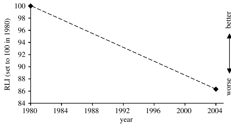
Figure 6. A preliminary Red List Index for all amphibian species for 1980–2004 (retrospectively assessed; n=496 genuine status changes/2225 species in categories extinct in the wild to near threatened, in at least one assessment; 1294 data deficient/5709 extant species).
