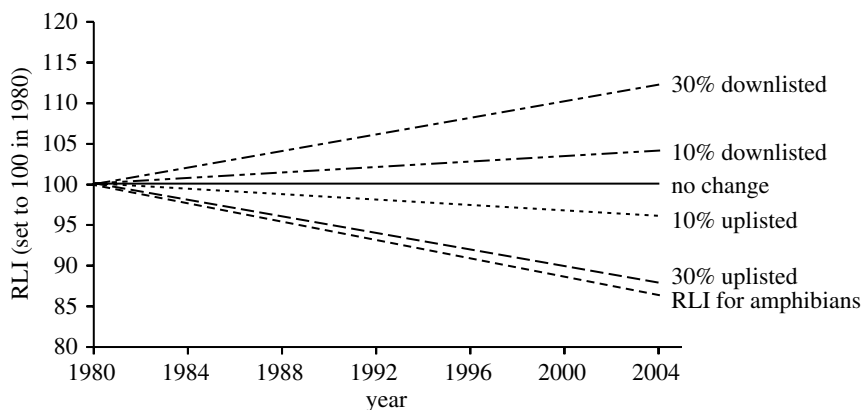
Figure 7. A preliminary Red List Index for all amphibian species for 1980–2004 (retrospectively assessed; n=496/2225 species), with hypothetical indices showing trends if zero species had changed category, and if 10 or 30% of species in the categories from near threatened to critically endangered had been up-listed to a higher category of threat or down-listed to a lower category of threat over the period.
