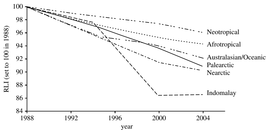
Figure 4. Red List Indices for birds for 1988–2004 in different biogeographic realms. Sample sizes: Afrotropical = 41 genuine status changes/394 species in categories extinct in the wild to near threatened, in at least one assessment; Indomalay = 100/585, Nearctic = 9/92, Neotropical = 49/834, Australasian/Oceanic = 53/614, Palearctic = 34/238.
