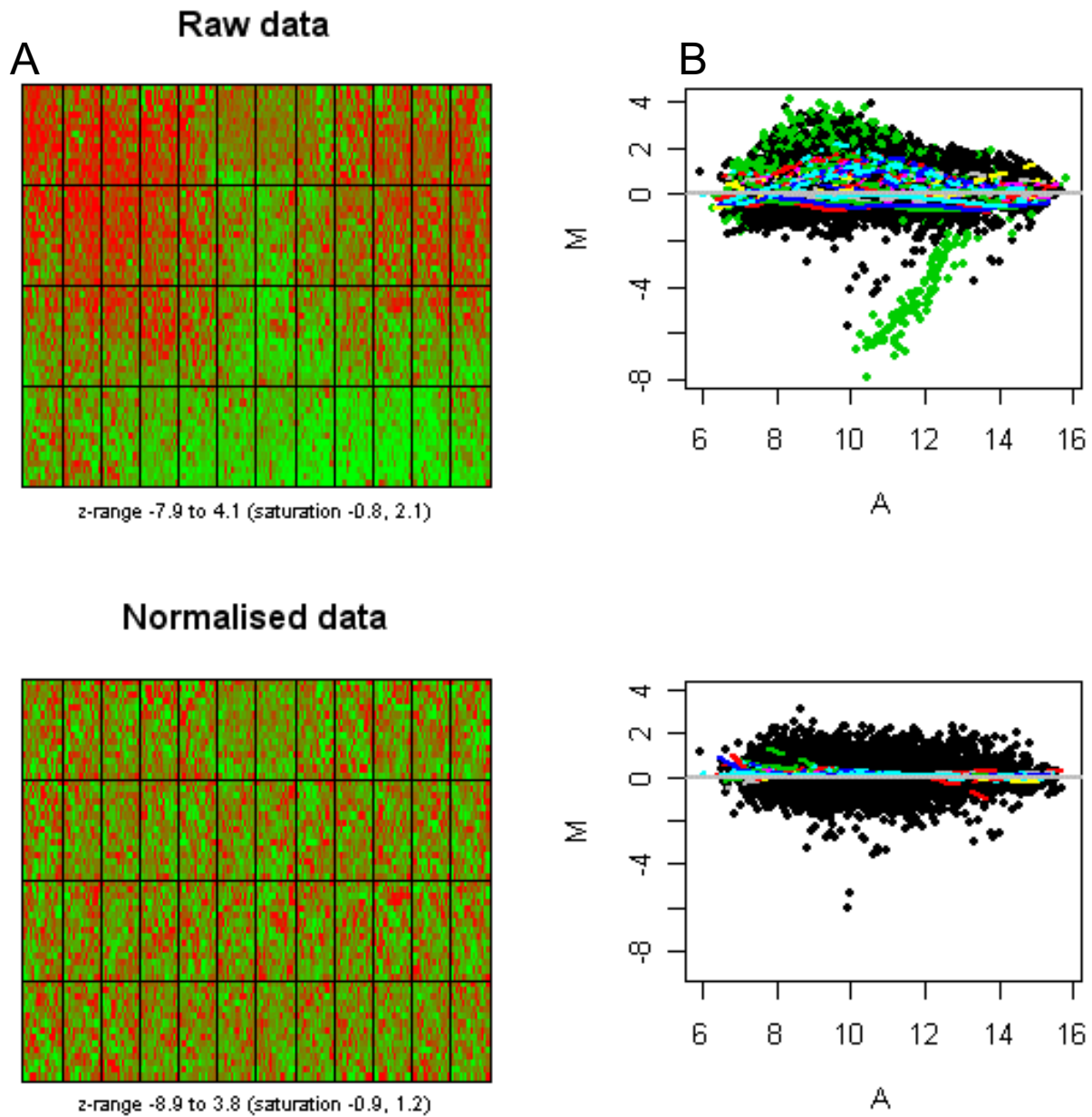
Figure 2 Representative spatial heat maps and M-A plots of raw and normalized data. A, spatial heat map for a representative microarray slide before and after normalization. The footnote gives the range of M values for the slide (z-range) and the range excluding the extreme 5% tails of the distribution of M values (saturation) which are excluded from the plot. B, M-A plots for the same representative microarray slide before and after normalization. Green spots denote control genes and the coloured lines represent the curve for each print tip.
