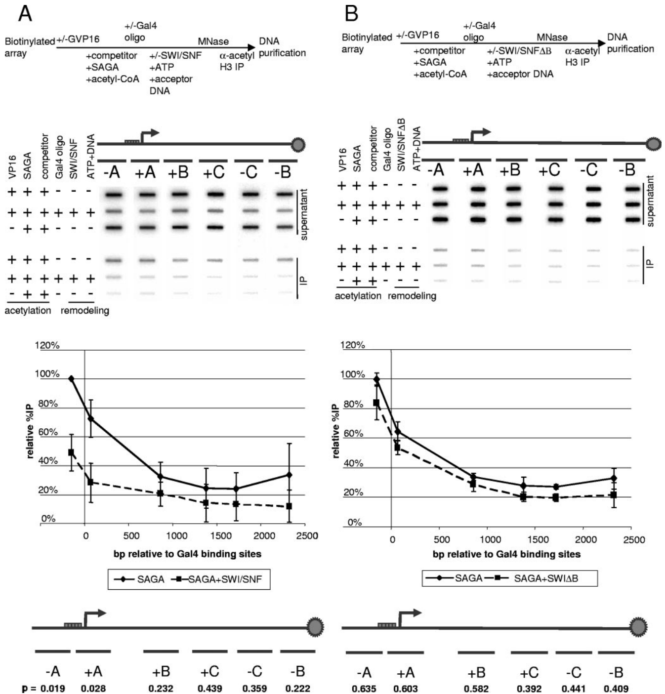
FIG. 4. The Swi2/Snf2 bromodomain is required for the transfer of acetylated histones. (A) SWI/SNF reduction of acetylated histone peak can occur without Gal4-VP16 targeting of this complex. Scanning in vitro ChIP analysis after SWI/SNF nucleosome displacement in the absence of activator Gal4-VP16. The experiment was previously described in Fig. 2. The template is bound to activator Gal4-VP16, acetylated by SAGA with competitor chromatin, and activator is removed by Gal4 oligonucleotide competition. The array was then subjected to SWI/SNF nucleosome displacement and immunoprecipitated with an anti-acetyl H3 antibody. The graph depicts the loss of promoter-acetylated nucleosomes after SWI/SNF nucleosome displacement without activator. The %IP was normalized to the %IP at the -A probe. The solid line depicts the H3 acetylation profile along the template, while the dashed line corresponds to the effect of SWI/SNF nucleosome displacement on the H3 acetylation profile. (B) Scanning in vitro ChIP analysis after activator is removed and SWI/SNF bromodomain mutant treatment. The experiment was as described in Fig. 2. Gal4-VP16 targeted SAGA acetylation at the promoter nucleosomes using competitor chromatin. The activator is removed by Gal4 oligonucleotide competition, and the array is subjected to nucleosome displacement by the bromodomain mutant complex, followed by IP with an anti-acetyl H3 antibody. The graph depicts the loss of promoter-acetylated nucleosomes after nucleosome displacement by the Swi2/Snf2 bromodomain mutant complex. The %IP was normalized to the %IP at the -A probe. The solid line depicts the H3 acetylation profile along the template, and the dashed line corresponds to the effect of Swi2/Snf2 bromodomain mutant on the H3 acetylation profile. A Student t test was used to determine the statistical significance of the difference in the acetylation profile before and after SWI/SNF treatment. The P values for the t test are given below each segment of the array.
