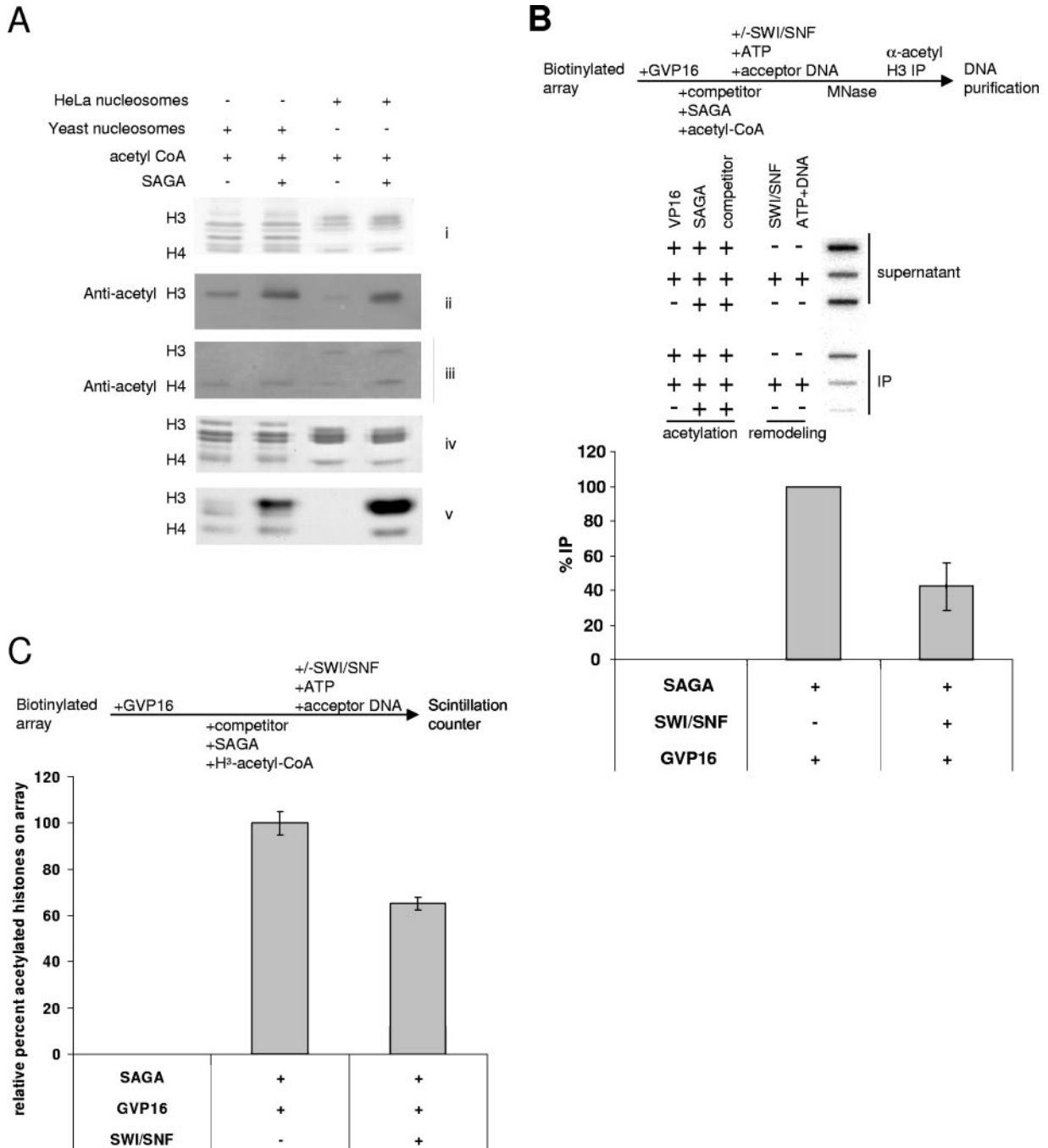
FIG. 1. SWI/SNF reduces the amount of acetylation detected on immobilized nucleosomal arrays. (A) Yeast and HeLa nucleosomes are equivalent substrates for yeast SAGA acetylation. Yeast or HeLa nucleosomes were incubated with acetyl-CoA and/or yeast SAGA. (i) As a loading control, half the reaction was silver stained. (ii and iii) The nucleosomes were immunoblotted with antibodies directed against anti-acetyl H3 and anti-acetyl H4, respectively. For fluorography, yeast or HeLa nucleosomes were incubated with H 3 -acetyl-CoA and/or yeast SAGA. (iv and v) As a loading control, half the reaction was Coomassie blue stained (iv) prior to electrophoresis, ENHANCE treatment, and fluorography (v). (B) SWI/SNF treatment causes a decrease in acetylation on the nucleosome array. Using competitor chromatin, the artificial activator Gal4-VP16 targets SAGA acetylation, and the array is subjected to SWI/SNF treatment, with acceptor DNA and ATP. After nucleosome displacement, the supernatant is removed, and the array is MNase digested and immunoprecipitated with an anti-acetyl H3 antibody. The immunoprecipitated nucleosomes are subjected to DNA purification and slot blotted onto nylon membrane, along with the supernatant. The membrane is probed with end-labeled full-length pG5E4T template. The %IP is the immunoprecipitated fraction divided by the sum of the immunoprecipitated fraction and the supernatant. In this case, the %IP was normalized to the %IP without SWI/SNF treatment. (C) SWI/SNF targets and displaces activator-targeted SAGA acetylation. The artificial activator Gal4-VP16 is bound to the immobilized nucleosomal array. After the addition of competitor, the array is acetylated with SAGA. The array is subjected to SWI/SNF nucleosome displacement with ATP and acceptor DNA, and the beads are counted on a scintillation counter. The loss of acetylation on the beads corresponds to nucleosomes displaced by SWI/SNF from the array. The change in acetylation on the array is expressed as the relative percent acetylated histones on the beads.
