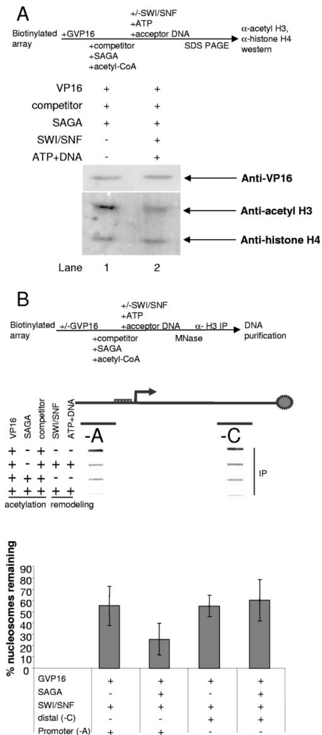
FIG. 3. Acetylated histones are preferentially lost after SWI/SNF nucleosome displacement. (A) The array is bound by activator Gal4-VP16 prior to the addition of competitor chromatin, followed by acetylation under competitive conditions with SAGA. After SWI/SNF nucleosome displacement, free histones are washed away, and the array is subjected to immunoblotting with an anti-VP16 antibody, an anti-acetyl H3 antibody, and an anti-histone H4 antibody. (B) Scanning in vitro ChIP assay with histone H3 antibody. The array is subjected to nucleosome displacement and ChIP as described in Fig. 1B. The membrane is hybridized to a promoter specific probe (-A) and a distal
