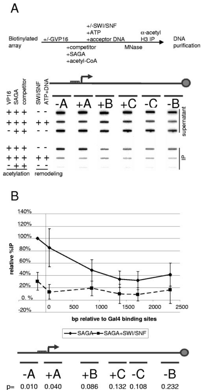
FIG. 2. Nucleosome displacement suppresses the SAGA acetylation peak. (A) Scanning in vitro ChIP assay, with the relative positions of the probes for the pG5E4T array indicated. The array was subjected to nucleosome displacement and ChIP as described in Fig. 1B. The membrane was hybridized to a series of labeled probes shown in the diagram. The positions of the probes relative to the HindIII restriction enzyme site are also indicated on the diagram. The blots are shown below each corresponding probe. (B) The SAGA acetylation peak is suppressed by SWI/SNF. The %IP was normalized to the %IP at the -A probe, which is upstream of the Gal4 binding sites and the E4 promoter. The solid line depicts the H3 acetylation profile along the template, while the dashed line corresponds to the effect of SWI/SNF nucleosome displacement on the H3 acetylation profile. A Student t test was used to determine the statistical significance of the difference in the acetylation profile before and after SWI/SNF treatment. The P values for the t test are given below each segment of the array.
