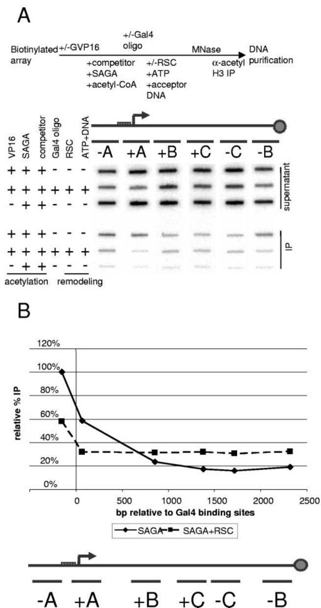
FIG. 5. RSC nucleosome displacement suppresses the SAGA acetylation peak. (A) RSC reduction of acetylated histone peak can occur without Gal4-VP16 targeting of this complex. Scanning in vitro ChIP analysis was performed after RSC nucleosome displacement in the absence of activator Gal4-VP16. The experiment was as described in Fig. 2. The template is bound to activator Gal4-VP16, acetylated by SAGA with competitor chromatin, and the activator is removed by Gal4 oligonucleotide competition. The array was then subjected to RSC nucleosome displacement and immunoprecipitated with an anti-acetyl H3 antibody. (B) The graph depicts the loss of promoter-acetylated nucleosomes after RSC nucleosome displacement without activator. The %IP was normalized to the %IP at the -A probe. The solid line depicts the H3 acetylation profile along the template, while the dashed line corresponds to the effect of RSC nucleosome displacement on the H3 acetylation profile. The graph shows the average of two independent experiments.
