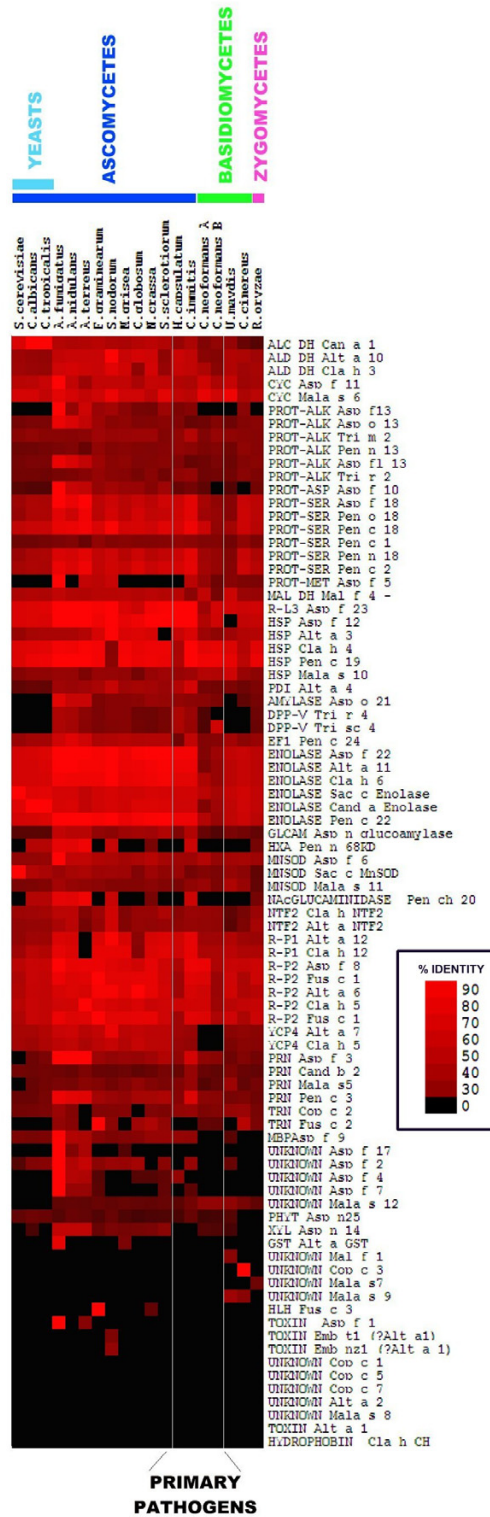
Figure 2 A Heat map showing homologies of fungal allergen genes to fungal genomes. The heat map was constructed from an MS excel file using Cluster and Treeview. Identities are coded by increasing colour saturation with bright red denoting the highest degree of identity.
