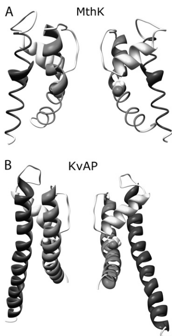
FIGURE 2 Side views of MthK and KvAP channels. A rotation around the hinge glycines (highlighted in the Corey-Pauling-Kultin mode) opens the intracellular channel mouths to different extents in the two channels.
