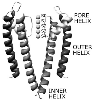
FIGURE 1 Side view of the KcsA channel. For clarity, only two subunits are shown. Five potassium ions are included in the SF at the binding sites S0–S4; numbering starts from the top (extracellular side).
