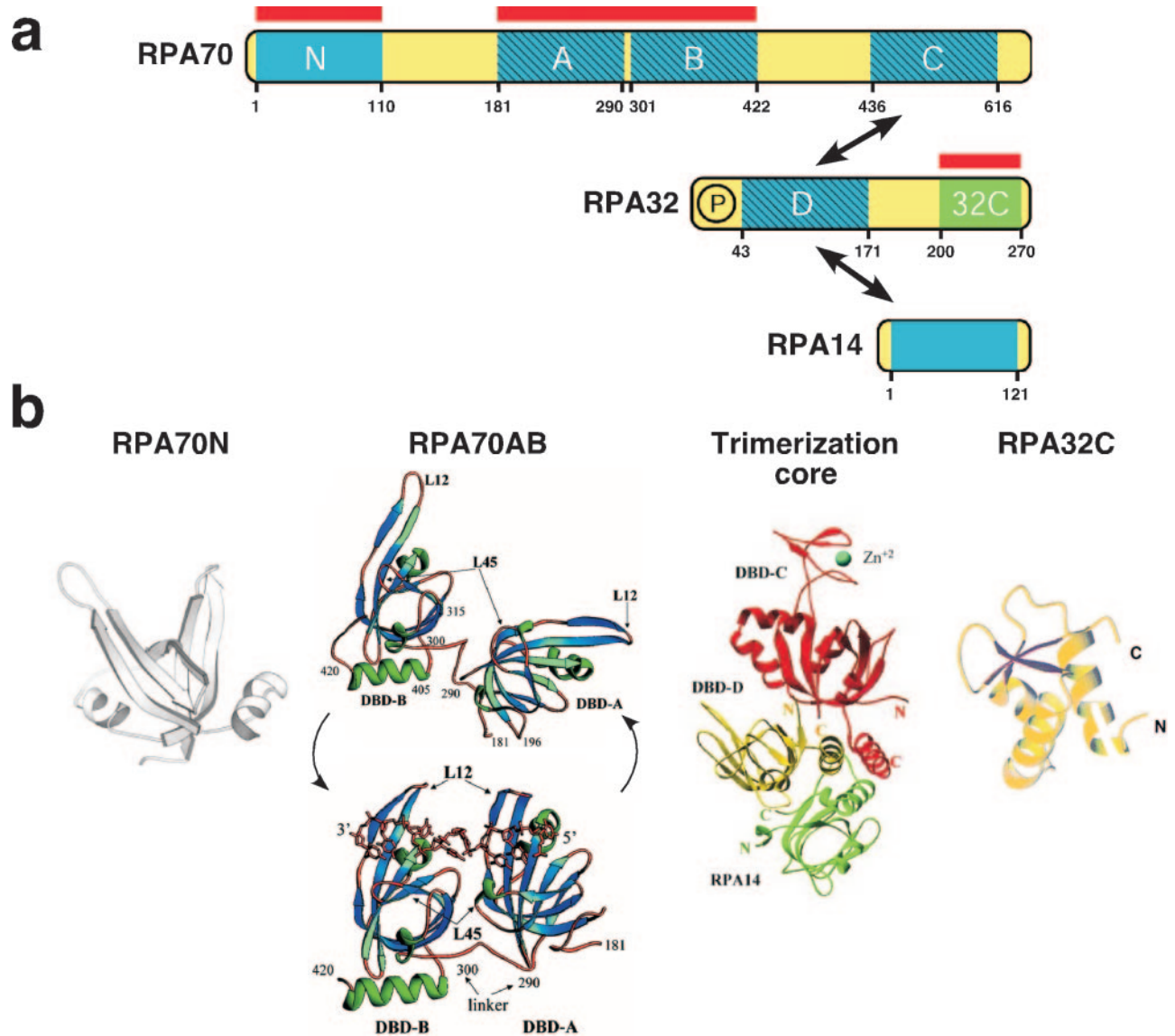
Figure 1. The modular structure of RPA. (a) Schematic diagram: arrows indicate intersubunit associations; protein-binding domains are denoted by red bars; ssDNA binding domains A–D by hatching; OB-folds by blue boxes; linkers by yellow boxes; winged helix by a green box; phosphoamino acid cluster by a circled P [adapted from (29) with permission]. (b) Structural models of RPA domains. [Reprinted from (20,24,25,55) with permission.]
