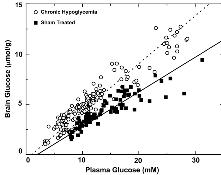
Fig. 3. Brain glucose concentrations as a function of plasma glucose levels in the sham-treated (solid squares) and chronically hypoglycaemic animals (open circles). The best fit of the ReMM model (eqn 2) to the measurements in the sham-treated group resulted in a relative maximum transport rate of T_{\max}/\text{CMR}_{\text{glc}} = 4.2 \pm 0.2 between the chronically hypoglycaemic group (dashed line), and the sham-treated group (solid line) T_{\max}/\text{CMR}_{\text{glc}} = 2.6 \pm 0.1 ( p < 0.0001 ).
