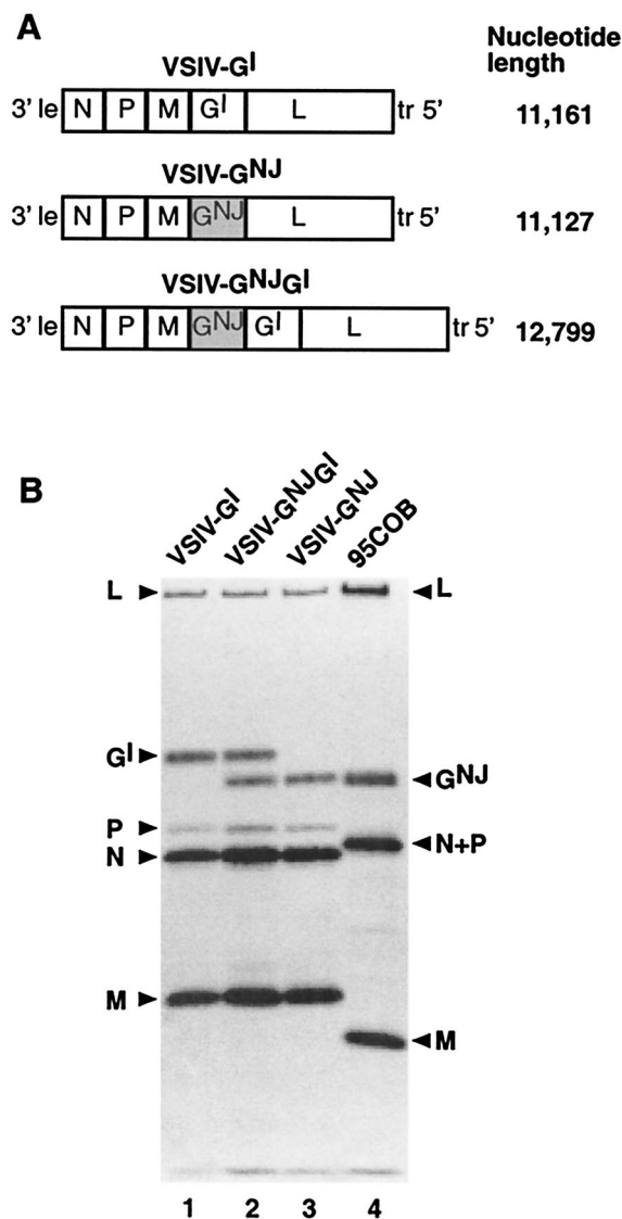
FIG. 1. (A) Schematic representation of recombinant VSV genomes. The negative-strand recombinant VSIV genomic RNAs indicating the gene order and expressed proteins are shown. VSIV leader (le), trailer (tr) and viral (N, P, M, G I , and L) genes are represented. G NJ refers to the glycoprotein gene from the VSNJV field isolate 95COB (shaded boxes). The lengths of the genomes are shown on the right. (B) Viral proteins incorporated in virus particles. Virions were labeled with [ 35 S]methionine and purified by centrifugation through 10% sucrose, and the virion proteins were analyzed by sodium dodecyl sulfate-polyacrylamide gel electrophoresis. The infecting viruses are indicated above the lanes, and synthesized proteins are indicated on the left for the recombinant VSIV viruses and on the right for 95COB.
