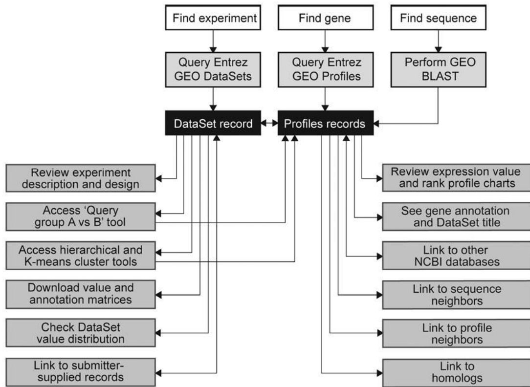
Figure 4. Schematic overview of the query workflow, and how the various features and tools are interlinked.
