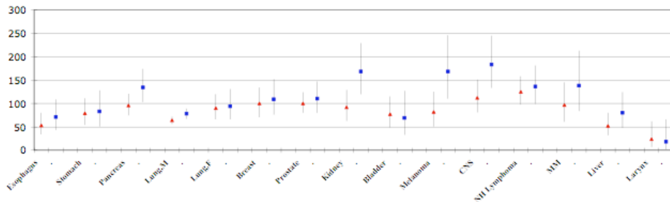
Figure 1 Comparison of SMRs and PCMRs. Comparison of SMRs (triangles) for selected cancers from Table 2 in ref. 6 with PCMRs (squares) for manufacturing plant decedents. The vertical lines are the Upper and Lower 95% Confidence Limits of the SMRs and PCMRs. All data are for males and females combined except for prostate, breast and lung cancer; SMRs are for the years 1965–1999 and for those who died 15 or more years since first employment. PCMRs are for the years 1969–2001 and for those who died ten or more years since first employment.
