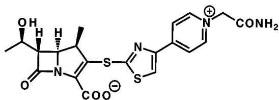
FIG. 1. Chemical structure of SM-17466.
