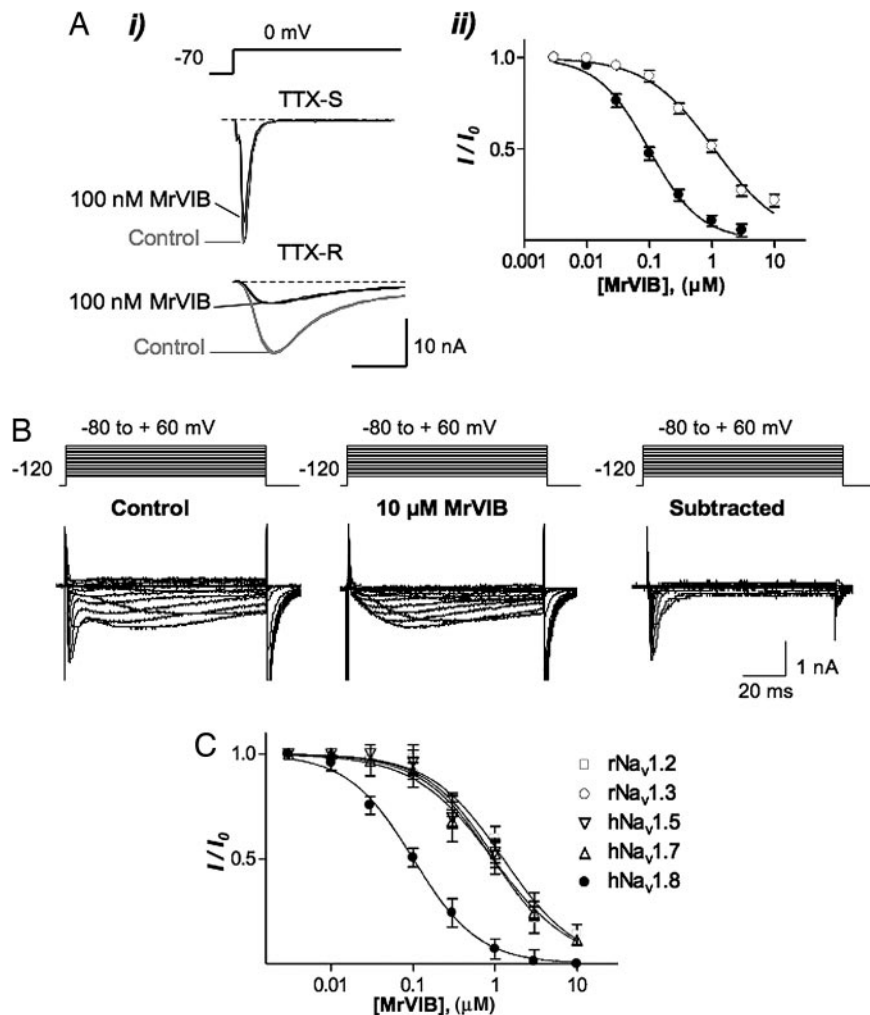
Fig. 1. MrVIB selectively blocks a TTX-R current in DRG and Na v 1.8. (A) Inhibition of transient TTX-S and TTX-R Na + currents in rat DRG neurons by MrVIB. (A i ) Superimposed depolarization-activated TTX-S and TTX-R Na + currents in the absence (control) and presence of 100 nM MrVIB. The TTX-S Na + current was recorded from a large ( \approx 45 - \mu m -diameter) DRG neuron that exhibited a Na + current with fast activation and inactivation kinetics that was 95% inhibited by 300 nM TTX, whereas the TTX-R Na + current was recorded from a small ( \leq 25 - \mu m -diameter) neuron in the presence of 300 nM TTX. (A ii ) Comparison of toxin inhibition of TTX-R (●) versus TTX-S (○) Na + current. The half-maximal inhibitory concentration ( IC_{50} ) was 98 nM ( n = 6 ) for the TTX-R Na + current and 1.1 \mu M ( n = 6 ) for the TTX-S Na + current. (B) MrVIB has no effect on the persistent TTX-R Na + current in rat DRG neurons. Currents obtained from a DRG neuron containing both slowly inactivating (Na v 1.8) and persistent (Na v 1.9) TTX-R Na + currents in the absence (control) and presence of 10 \mu M MrVIB. TTX (300 nM) were present throughout the experiment. Neurons were held at -120 mV and depolarized to voltages ranging from -80 to +60 mV in 10-mV increments, generating slowly inactivating and persistent Na + currents of different amplitude. MrVIB at 10 \mu M completely inhibited the slowly inactivating TTX-R Na + current, although leaving the persistent TTX-R Na + current intact. Subtraction of the Na + currents recorded in presence of MrVIB from control Na + current resulted in typical Na v 1.8 currents, further demonstrating that MrVIB at 10 \mu M completely inhibits Na v 1.8 but not Na v 1.9. (C) Concentration–response relationship for MrVIB inhibition of different VGSC subtypes expressed in Xenopus oocytes. The IC_{50} for MrVIB was 102 nM for human (h)Na v 1.8 and \approx 1 \mu M for rat (r)Na v 1.2, rNa v 1.3, hNa v 1.5, and hNa v 1.7 ( n = 3 –6). I represents the maximal Na + current amplitude recorded in the presence of MrVIB at various concentrations, and I_0 represents the maximal Na + current obtained in the absence of toxin. Only oocytes that expressed VGSC currents >200 nA were used in this study. For comparison, MrVIB has been shown to inhibit the muscle-type VGSC Na v 1.4 with an IC_{50} value of 222 nM (MrVIA showed a comparable potency of 265 nM) (17).
