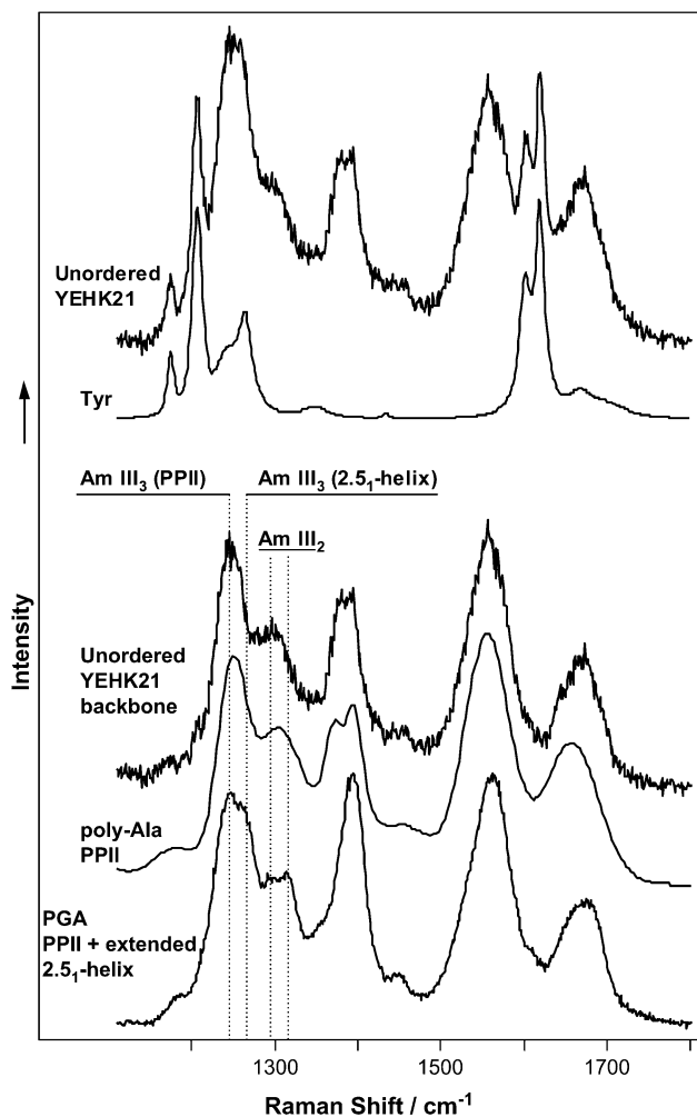
FIGURE 8 DUVRR spectra of unorderd polypeptides. (Top to bottom) The 197-nm excited room-temperature Raman spectrum of YEHK21 melted at 125°C and the Raman spectrum of tyrosine; the Raman spectrum of melted YEHK21 backbone obtained as a difference between the spectrum of melted YEHK21 and the spectrum of tyrosine; the 204-nm DUVRR spectrum of 20-amino acid mainly alanine peptide adopted from Lednev et al. (58), previously reported (59) to be dominated by PPII conformation; the 197-nm DUVRR spectrum of PGA adopting PPII and extended 2.5 1 -helix conformations (59).
