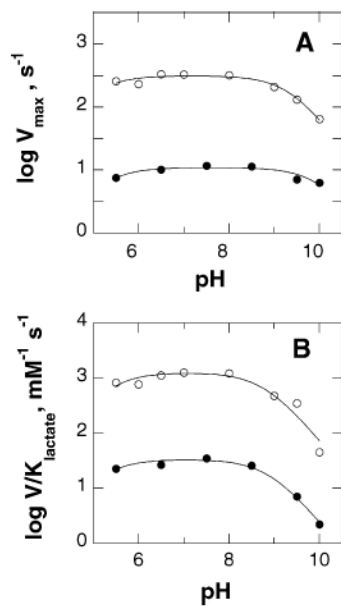
Figure 1. pH dependence of wild-type and Y254F flavocytochromes b_2 . Initial rates were determined with ferricyanide as the electron acceptor as described in Experimental Procedures. Panel A shows the V_{\max} profile and panel B the V/K_{\text{lactate}} profile for the wild-type (○) and for the Y254F (●) enzymes. The lines are fits of the data to eq 3. The data for the wild-type enzyme are from ref 21.
