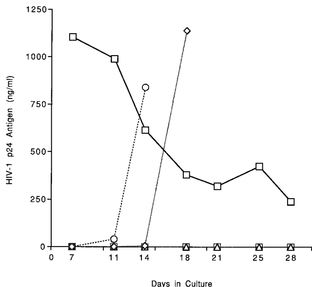
FIG. 3. Inhibition of HIV-1 replication by limited exposure (3 days) to PRO 2000 at 10 ( \diamond ), 20 ( \circ ), 40 ( \triangle ), or 100 ( \square ) \mu\text{g/ml} following simultaneous infection of H9 cells. \square , infected control. For the 40- \mu\text{g/ml} preparation, one of two culture wells showed viral breakthrough by day 18, and the second culture well showed suppression of virus through day 28 in culture.
