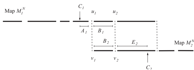
Fig. 1. The distance between optical map midpoints. The distance between maps M_1^N and M_2^N is given by the distance between map centers. In this case, dist(M_1^N, M_2^N) = dist(C_1, C_2) = (-1)^{(u_1=C_1, v_2=C_2)} \times (A_1 + (B_1 + B_2)/2 + E_2) , where u_1 represents the closest to C_1 matching site of the largest alignment block ( u_1, u_2; v_1, v_2 ) that does not contain center points C_1 and C_2 .
