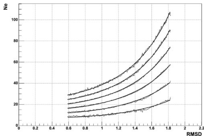
Figure 2. Quadratic exponent fit (solid line) of dependencies \mu , \mu + \sigma , \mu + 2\sigma , \mu + 3\sigma , \mu + 4\sigma , \mu + 5\sigma (dashed line).
