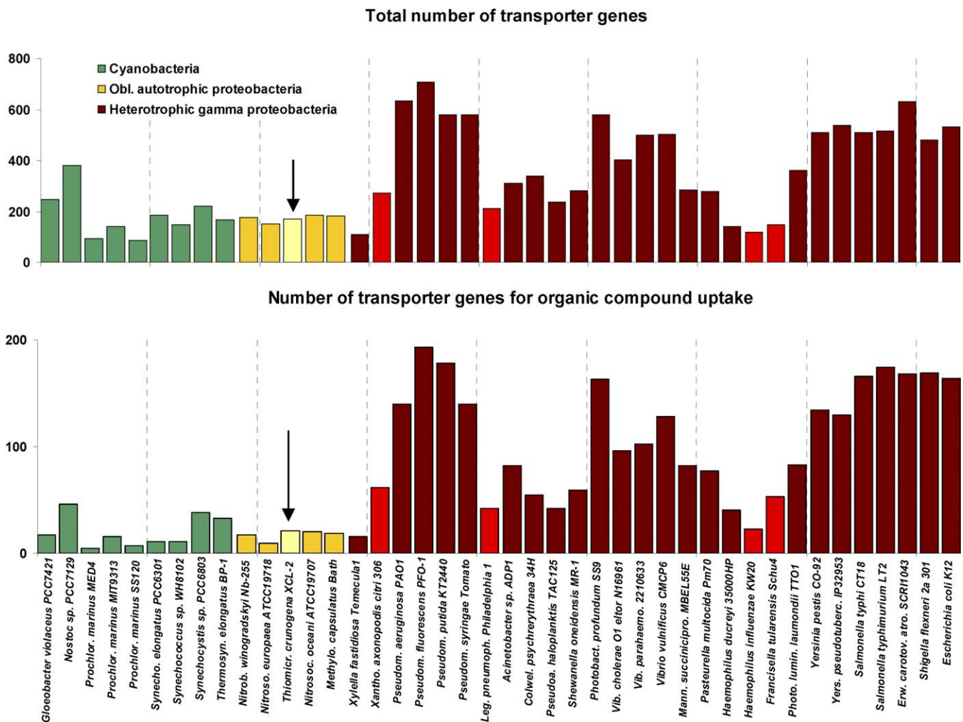
Figure 5. Transporter Gene Frequencies within the Genomes of Thiom. crunogena XCL-2 (Arrow) and Other Proteobacteria Nitrob. winogradskyi ( Nitrobacter winogradskyi ) is an alphaproteobacterium, Nitros. europaea ( Nitrosomonas europaea ) is a betaproteobacterium, and Nitrosoc. oceani ( Nitrosococcus oceani ) and Methylo. capsulatus ( Methylococcus capsulatus ) are gammaproteobacteria. Bars for intracellular pathogens are lighter red than the other heterotrophic gammaproteobacteria. DOI: 10.1371/journal.pbio.0040383.g005
