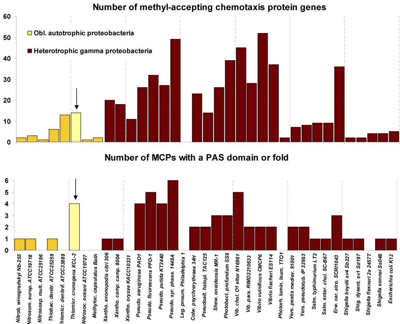
Figure 9. Numbers of MCP Genes in Thiom. crunogena XCL-2 and Other Proteobacteria Thiom. crunogena is marked with an arrow. DOI: 10.1371/journal.pbio.0040383.g009
