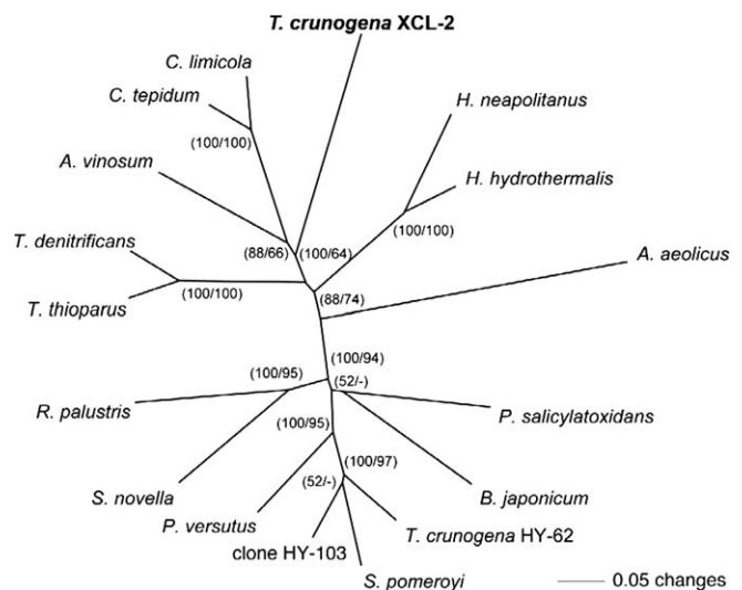
Figure 4. Phylogenetic Relationship of Thiom. crunogena XCL-2 SoxB to Sequences of Selected Bacteria
