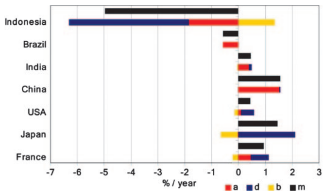
Fig. 3. Depicted during 1990–2005 in each of seven countries are the rate of change of total above-ground biomass ( m ) (upper bars) and (lower bars), the contributions of changing area ( a ), growing stock density ( d ), and biomass ( b ) per volume of growing stock that summed to change ( m ) (source, ref. 4).
