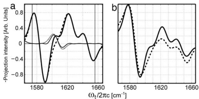
Fig. 5. Traces of 2D IR correlation spectra. (a) Least-squares fit to the 12 \text{ cm}^{-1} -wide trace along the \omega_t axis of the heterodimer (G_{79}^* + G_{79}^{**}) - 0.25G_{79}^{**} as described in the text (thick solid line), the fit omitting the cross-peak (thick dashed line), the difference between the solid and the dashed line (thin solid line), and the cross-peak response from least-squares-fitting the whole spectral region between the two vertical lines (thin dotted line). (b) Comparison between the ^{13}\text{C}=\text{18O} trace of G_{79}^* + G_{79}^{**} (solid line) and the control sample G_{94}^* + G_{79}^{**} (dashed line).
