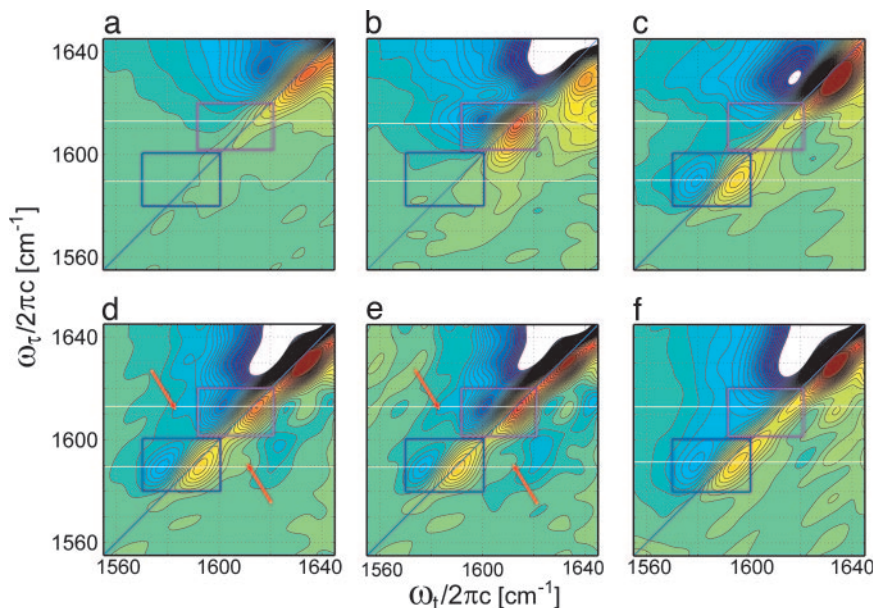
Fig. 4. The 2D correlation spectra of GpA TM homodimers G_{79} (a), G_{79}^* (b), and G_{79}^{**} (c); heterodimers G_{79}^* + G_{79}^{**} (d) and (G_{79}^* + G_{79}^{**}) - 0.25G_{79}^{**} (e); and control sample G_{94}^* + G_{79}^{**} (f) in 5% SDS. The ^{13}\text{C}=\text{16O} and ^{13}\text{C}=\text{18O} isotopomer diagonal regions are highlighted by rectangular boxes, and the arrows point to the cross-peaks.
