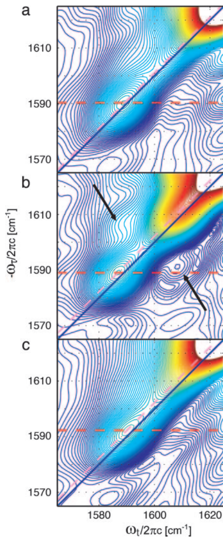
Fig. 3. The rephasing magnitude spectra of homodimer G_{79}^{**} (a), heterodimer G_{79}^* + G_{79}^{**} (b), and control heterodimer G_{94}^* + G_{79}^{**} (c). The horizontal line indicates the ^{13}\text{C}=\text{O} peak position, and the diagonal line is a slice of the spectrum shown in Fig. 2d. The arrows point to the cross-peaks.
