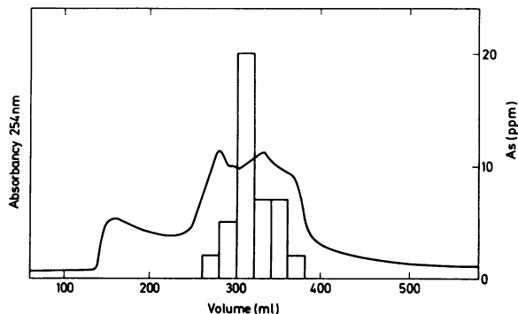
FIGURE 2. Molecular gel filtration of glue water (cod): (—) absorption at 254 nm; (□) concentration of arsenic. Data of Lunde (23).
