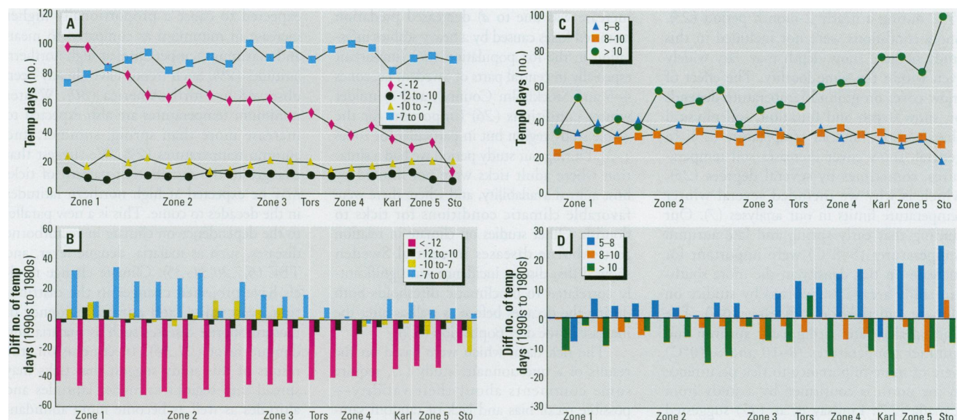
Figure 3. The climate in the various study districts and zones in the 1980s and the differences between the 1990s and the 1980s. Abbreviations: Karl, Karlstad Meteorological Station; Sto, Stockholm Meteorological Station; Tors, Torsby Meteorological Station. The average number of days during 3 years in the early 1980s with temperatures (temps) below, in between, or above bioclimatic thresholds of interest for tick distribution and density in each of the 20 study districts are shown for winter (A) and spring, summer, and autumn (C); the most northern study districts are to the left and the most southern are to the right along the x-axis. The difference between the 1990s and the 1980s in the average number of days for each temperature variable are shown for winter (B) and spring, summer, and autumn (D); study districts with increasing tick density and changes in tick occurrence on cats and dogs in the 1990s are shown over time from left to right along the x-axis.
