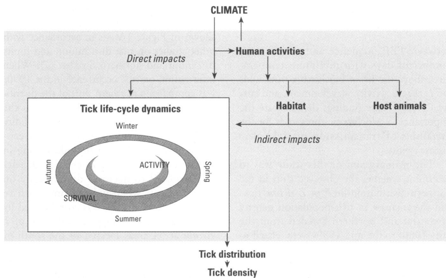
Figure 2. Schematic illustration of direct and indirect climatic impacts on tick distribution and population density.
