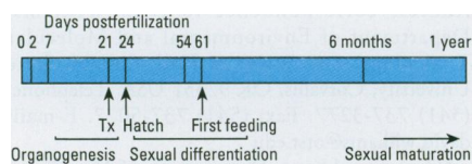
Figure 1. Timeline of rainbow trout sexual development. a DPF, days postfertilization: 0–2 DPF, egg hardening (early embryogenesis); 7–21 DPF, organogenesis (eye pigmentation indicates development stage/rate); 21 DPF, injection (Tx); 24–28 DPF, hatch (period of high stress and mortality); 54 DPF, yolk-sac absorption (assimilation and redistribution of yolk products); 61 DPF, first feeding (period of high stress and mortality); 4–6 months, gonads become recognizable; 1–2 years, gonadal maturation and spawning.
