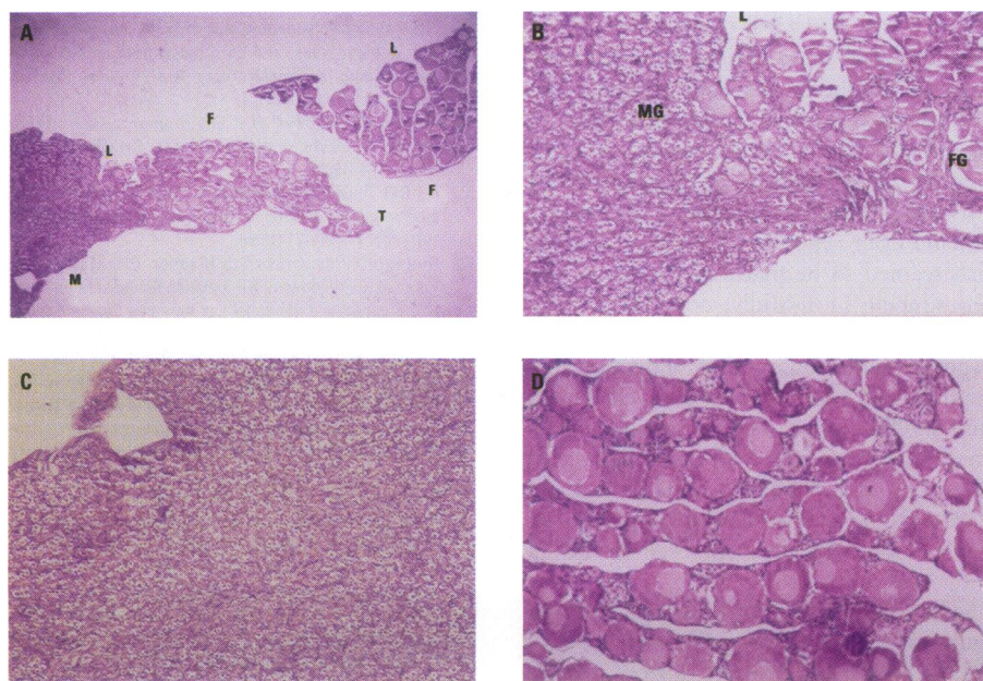
Figure 3. Gonad of 6-month-old morphologic female rainbow trout treated with 160 mg/kg o,p' -DDE in ovo (experiment 1). Abbreviations: T, tear in gonad, probably not related to treatment; F, characteristic female gonad structure; M, characteristic male gonad structure; L, lamellae structures characteristic of female gonads. (A) The gonad appears to have distinct female and male portions, with no apparent mixing of germ cells except around the transition boundary shown here (8 \times magnification). (B) High magnification (132 \times ) of the transition point between the female and male gonad structures. Note the distinct membrane characteristic of female lamellae (L) (appears to be a final lamellar structure rather than a tear in the gonad, as characterized by the intact membrane); a typical female germ cell (FG) at 6 months of age; and the typical cluster arrangement of male germ cells (MG) at this stage of development. This is the only portion of the gonad where male and female germ cells can be seen together. (C) Male portion of the gonad representative of a normal male gonad in fish of this age (32 \times magnification). (D) Female portion of the gonad representative of normal female gonad in fish of this age (32 \times magnification).
