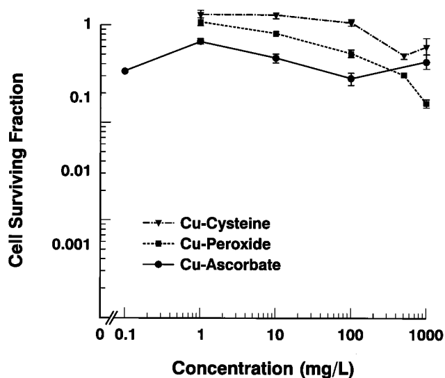
FIG. 4. Survival of cells exposed to Cu(II) at 1 mg/liter and various concentrations of cysteine, hydrogen peroxide, or ascorbic acid. The conditions used to treat cells, which were identical to those used to treat HSV in the experiment whose results are presented in Fig. 3, are described in Materials and Methods and in the legend to Fig. 2. The average \pm standard error (when they extend beyond the symbols) of four experiments is displayed.
