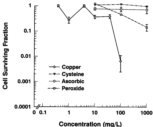
FIG. 2. Survival of Vero cells after treatment with different concentrations of Cu(II) or reducing agents. Cells were incubated with either cupric chloride, ascorbic acid, hydrogen peroxide, or cysteine at concentrations indicated on the x axis for 30 min at 21°C as described in Materials and Methods. After treatment, the cells were rinsed, trypsinized, resuspended in fresh medium, seeded in petri dishes, and incubated for 12 to 14 days at 37°C under 5% CO 2 . The number of colonies from cells surviving treatment relative to the number of colonies in untreated controls is displayed (means \pm standard error [when extending beyond symbols] from four independent experiments).
