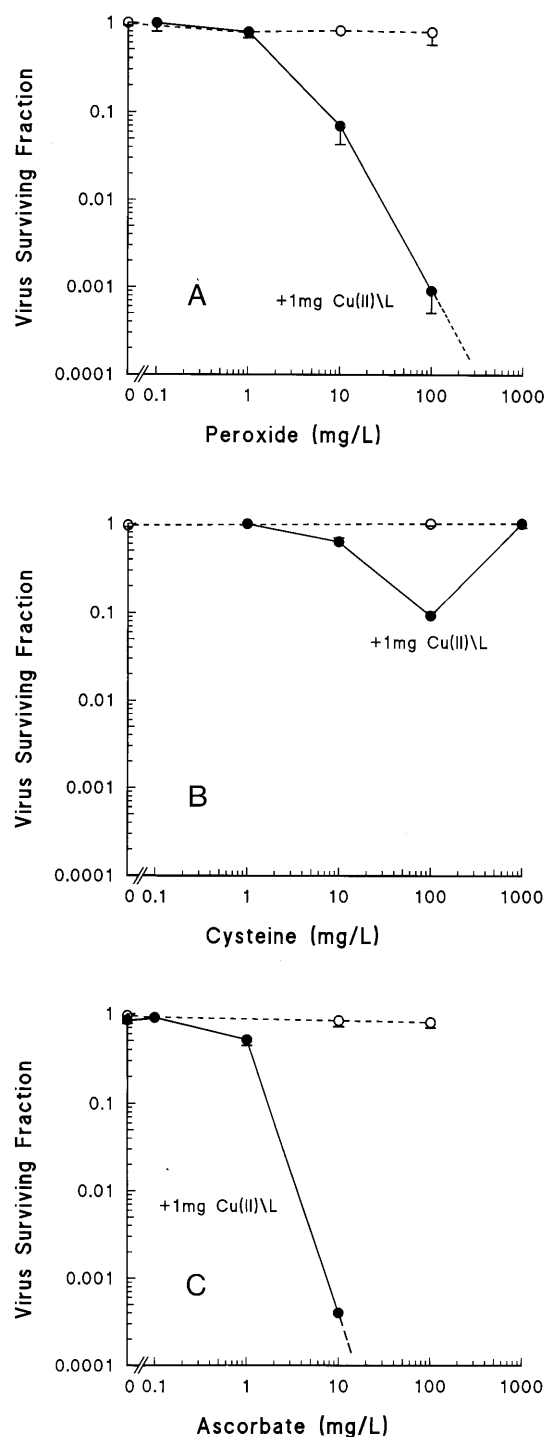
FIG. 3. Inactivation of HSV after exposure for 30 min at 21°C with 1 mg of Cu(II) per liter and different concentrations of hydrogen peroxide (A), cysteine (B), or ascorbic acid (C). Survival of HSV treated with the reducing agents in the absence of copper is indicated by open circles linked by dashed lines. Mean values from at least three independent experiments are presented; standard errors are shown as error bars when they extend beyond the datum symbols.
