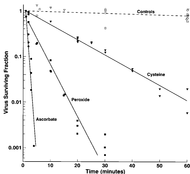
FIG. 5. Inactivation kinetics of HSV at 21°C by 1 mg of Cu(II)/liter and 100 mg of either cysteine, hydrogen peroxide, or ascorbate per liter. Data on the survival of HSV exposed to Cu(II) alone (open diamonds) or to each of the reducing agents (open triangles, squares, and circles, respectively) are included as controls.
