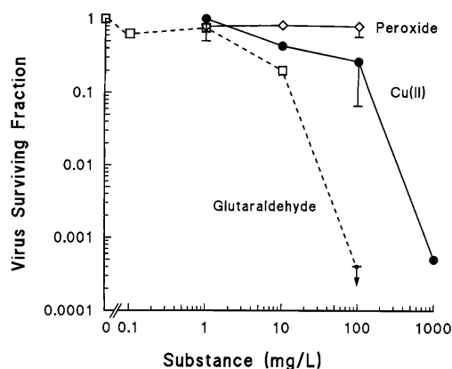
FIG. 1. Survival of HSV after treatment for 30 min at 21°C with different concentrations of Cu(II), hydrogen peroxide, or glutaraldehyde. Mean values from at least three independent experiments are presented; standard errors are shown as error bars when they extend beyond the datum symbols.
