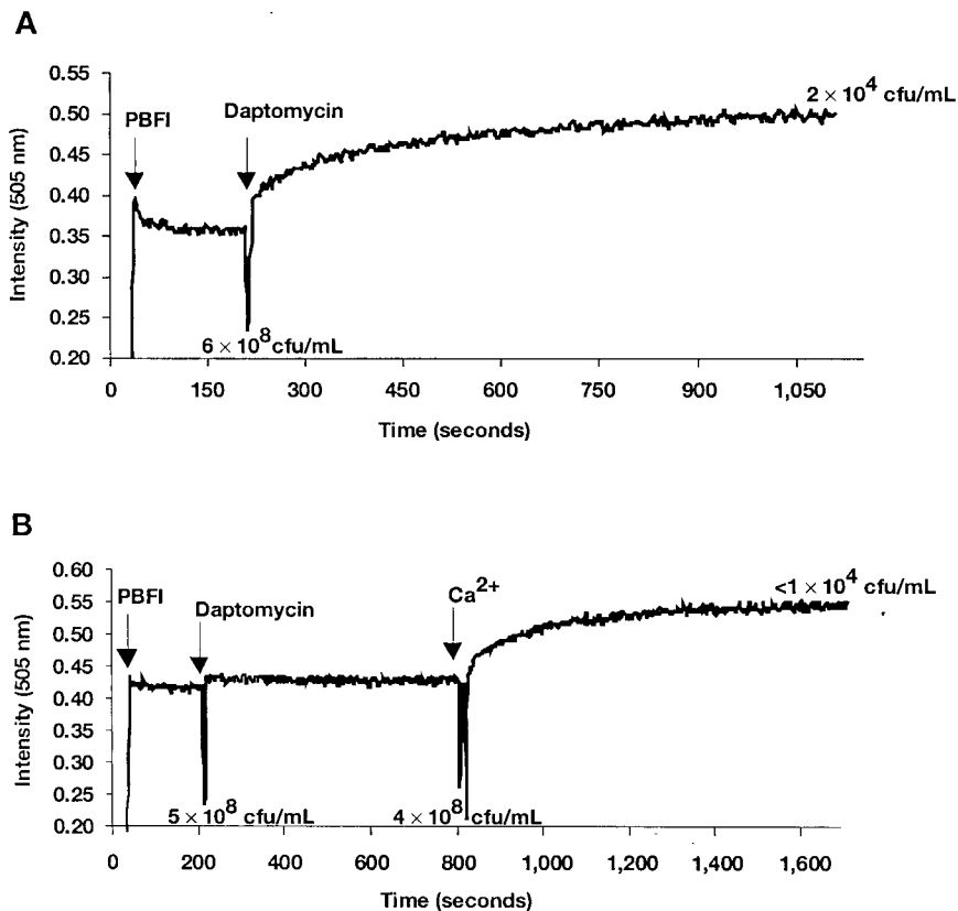
FIG. 5. Daptomycin triggers potassium release from S. aureus . (A) PBFi ( 1 \mu\text{M} ) and daptomycin ( 5 \mu\text{g/ml} ) were added to S. aureus in HEPES-glucose solution containing 1 \text{ mM} \text{CaCl}_2 at the indicated time points. (B) PBFi ( 1 \mu\text{M} ), daptomycin ( 5 \mu\text{g/ml} ), and \text{Ca}^{2+} ( 50 \text{ mg/liter} ) were added to S. aureus at the indicated time points. For both experiments, viable cell counts were determined at the indicated time points.
