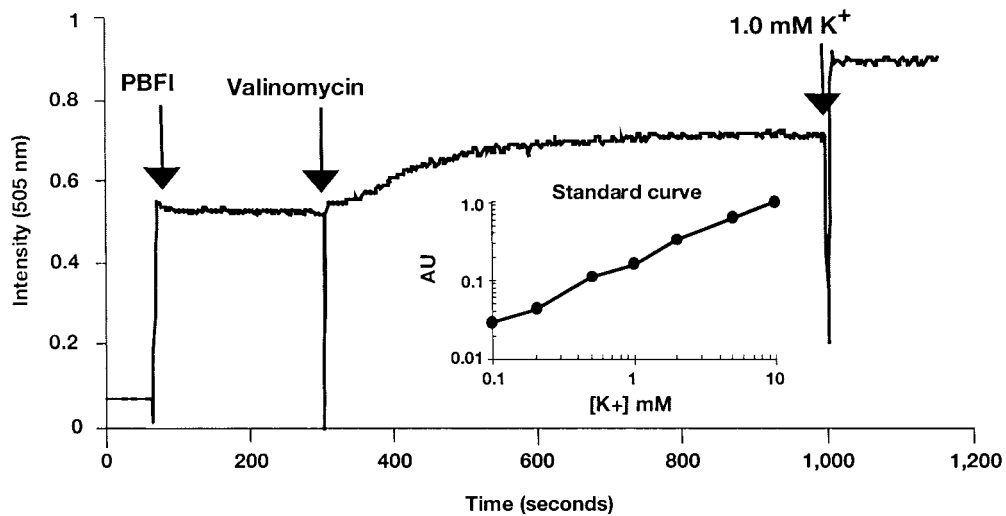
FIG. 4. Potassium release assay. PBFi ( 1 \mu\text{M} ), valinomycin ( 10 \mu\text{g/ml} ), and KCl ( 1 \text{ mM} final concentration) were added at the indicated time points to S. aureus in HEPES-glucose solution. AU, arbitrary unit.
