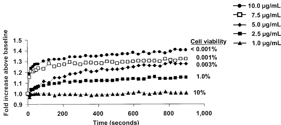
FIG. 6. Bactericidal activity and potassium release. Potassium release was triggered by the addition of 1 mM CaCl 2 . Data were normalized to the pre-calcium addition baseline values. The cell viability determined 15 min after calcium addition is indicated for each daptomycin dose level.
