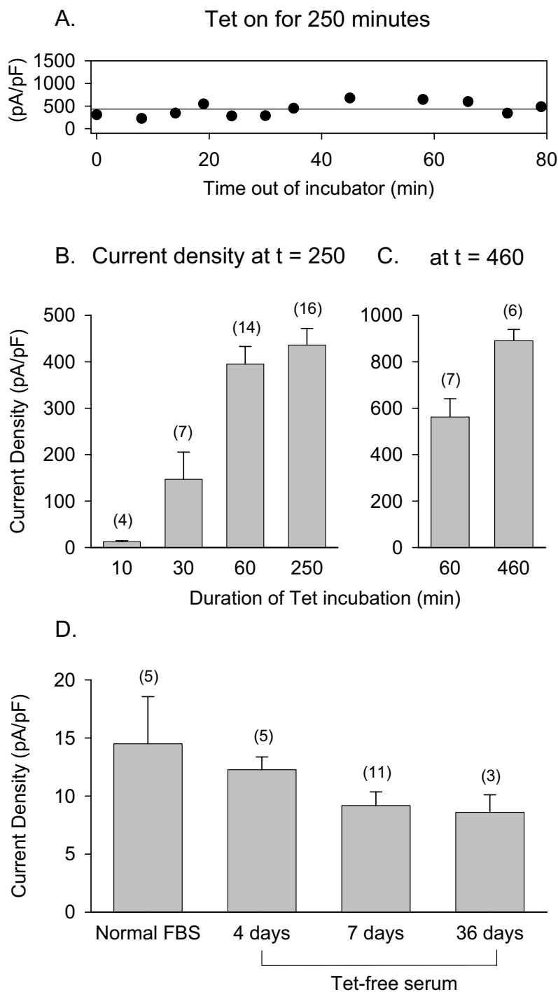
Figure 2 Long-term effects of Tet incubation on expression. (A) Cells were exposed to Tet in the incubator for 250 min, then removed from the incubator and kept in recording solution at room temperature. Recordings were made from a series of different cells over a period of 80 min to determine current density. The horizontal line is drawn at the mean density over the complete set of data. (B) Current density was determined at t = 250 min following the Tet incubation times shown on the abscissa. Values in parentheses denote the number of cells tested. (C) Current density was determined at t = 460 min following the Tet incubation times shown on the abscissa. (D) Cells were maintained in media containing no added Tet, plus either normal fetal bovine serum (FBS) or Tet-free serum for the number of days indicated on the abscissa.
