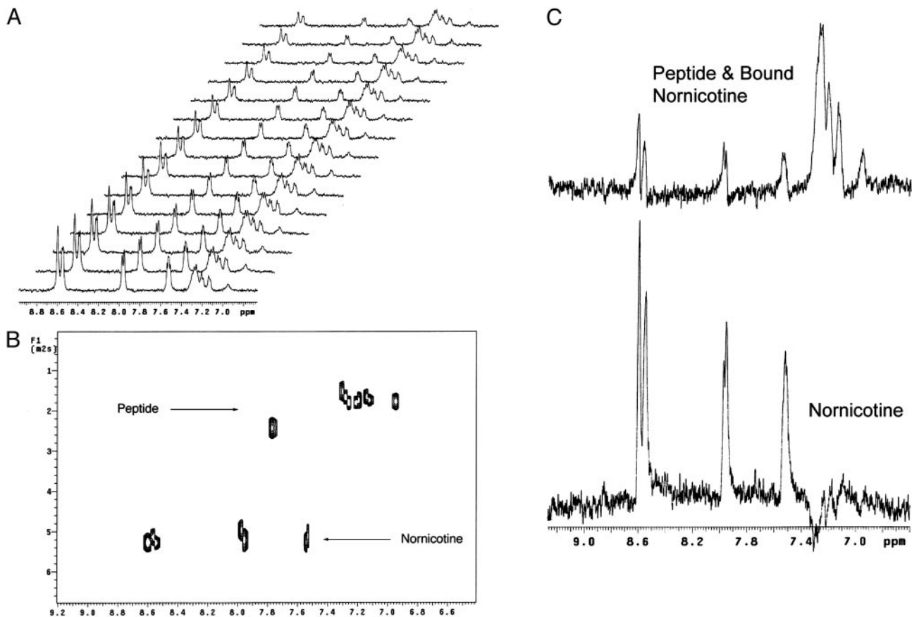
Fig. 3. Nornicotine glycation of A \beta 12–28 diffusion data. (A) Stacked plot of the obtained 1 H PFG-NMR spectra. (B) Pseudo 2D DOSY plot of diffusion data showing the observed differences in diffusion of nornicotine and amyloid peptide. It is important to note that the observed diffusion coefficient of nornicotine in this spectrum is the weighted average of both bound and unbound nornicotine. (C) Results of DECRA analysis of diffusion data showing two distinct populations of nornicotine, one bound to the peptide and the other free in solution.
