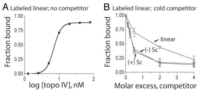
Fig. 2. Binding of Topo IV to linear, (+) supercoiled, and (-) supercoiled DNA. (A) Reactions containing linear ^{32}\text{P} -labeled pUC18 (1.3 nM) were incubated in binding buffer and the indicated concentration of Topo IV for 20 min at 30°C. The fraction of DNA bound to Topo IV was determined by filter binding. (B) Topo IV binding to linear ^{32}\text{P} -labeled pUC18 was competed against unlabeled linear ( \square ), (+) supercoiled (Sc) ( \triangle ), or (-) supercoiled (Sc) ( \square ) DNAs. Error bars are the standard deviations of duplicate experiments.
