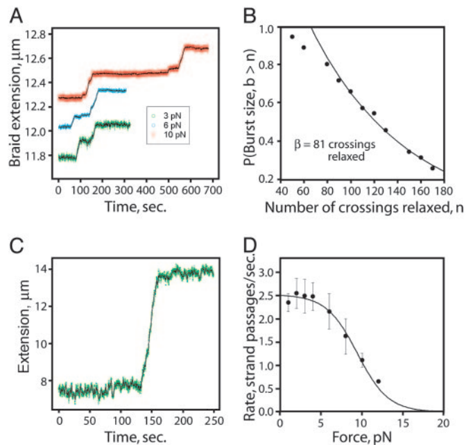
Fig. 6. Relaxation of braids by single Topo IV molecules. (A) Representative single-enzyme traces are shown for the indicated tensions and \sigma_{br} = -0.05 . (B) Processivity of unbraiding by single Topo IV molecules. The burst sizes ( b ) from 31 experiments are plotted as a cumulative histogram. Fitting of this histogram with a single exponential (neglecting undersampled short burst sizes) yields a decay constant ( \beta ) of 81 crossings. (C) Processive relaxation of a 44-kb (+) supercoiled DNA. A representative single Topo IV molecule supercoil relaxation experiment is shown for a DNA molecule ( \sigma = +0.03 ) held at 0.7 pN. Seventy-five crossings were relaxed in a single burst. (D) The effect of force on the rate of Topo IV unbraiding. The rates of relaxation were determined over each burst of activity and were fit to v(F) = v_0/[1 + (v_0/v_1)e^{(0.5F\Delta x)/(kT)}] (black line), where v(F) is the reaction velocity at force F , k is Boltzmann's constant, T is temperature, and v_0 is the rate of the force-independent kinetic step. For the force-dependent step, v_1 and \Delta x are, respectively, the unperturbed rate and the distance along the pulling axis to the transition state. ( v_0 = 2.5 catalytic cycles per sec, v_1 = 360 catalytic cycles per sec, and \Delta x = 4.3 nm.)
