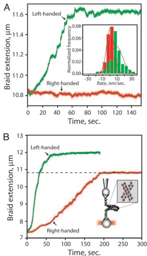
Fig. 4. Topo IV unbraiding of single DNA braids. (A) Preferential relaxation of left-handed braids. Topo IV activity was assayed by monitoring the extension of the braids held under constant tension (1 pN). Raw data are plotted in green (left-handed braid) and red (right-handed braid), and a 1-sec moving average is shown as a solid black line. (Inset) Histogrammed rates of unbraiding were calculated as \Delta Z/\Delta t for successive 5-sec windows in 10 independent runs each on right- and left-handed braids ( |\sigma_{br}| = 0.05 ). To avoid effects of limiting substrate, only those portions of the traces where |\sigma_{br}| > 0.02 were included. The mean unbraiding rate was 9 \pm 1.4 nm/sec for left-handed braids (green) and 0.3 \pm 0.3 nm/sec for right-handed braids (red). (B) Topo IV relaxation of high-density DNA braids for |\sigma_{br}| > 0.15 and 2 pN of tension. The first-order DNA braid folds into a plectonemic second-order superhelix, with DNA crossings possessing the opposite handedness of the first-order superhelix. Symbols are as in A. The dashed black line is the extension for |\sigma_{br}^{crit}| at 2 pN.
