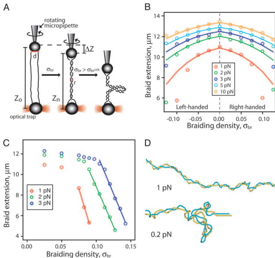
Fig. 3. Characterization of a single-molecule DNA braiding system. (A) Two nicked DNA molecules (solid black lines) are oriented between one bead on a rotating micropipette and another bead held in an optical trap. As braiding density, |\sigma_{\text{br}}| , increases, the length of the braid, Z , diminishes gradually until a critical braiding density is reached, |\sigma_{\text{br}}^{\text{crit}}| , at which point the braid buckles, forms a second-order plectonemic superhelix, and shortens much more dramatically with each introduced turn. (B) Shortening of braids as a function of braiding density. Braid length for \sigma_{\text{br}} < \sigma_{\text{br}}^{\text{crit}} can be approximated by a geometric model, Z_n = [Z_0^2 - (d + 2\pi rn)^2]^{1/2} , where Z_n is the extension of a braid with n turns, Z_0 is the maximal extension of the braid, d is the distance between points of attachment of the two DNA ends on each bead, and r is the effective radius of the braid. Braid extensions are shown over a range of \sigma_{\text{br}} and tensions. \circ , Experimental data; solid lines represent the fit to the model. (C) For |\sigma_{\text{br}}| > |\sigma_{\text{br}}^{\text{crit}}| , the braid compaction no longer obeys the simple model because of the buckling of the DNA braid into a plectonemic superhelix (second-order). The compaction of the braid in this regime is \approx 35 nm for each additional turn. (D) Monte Carlo simulations of DNA braids. Braids of two individual 3.5-kb DNA molecules (blue and yellow) with a \sigma_{\text{br}} = 0.05 , held under 1 pN or 0.2 pN of force, are shown.
