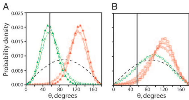
Fig. 5. Comparison of crossing segment juxtaposition angles in supercoiled, braided, and catenated DNA. (A) We define the angle of juxtaposed crossing segments ( \theta ) for braids in Fig. 1C and analogously for supercoiled and catenated DNA. The angular distribution between juxtaposed segments of DNA in simulated 3.5-kb (+) supercoiled ( \sigma = +0.05 , green circles) and (-) supercoiled ( \sigma = -0.05 , red circles) DNA under no force is plotted along with the angular distribution between juxtaposed segments of DNA in simulated left-handed ( \sigma_{br} = -0.05 , green triangles) and right-handed ( \sigma_{br} = +0.05 , red triangles) braids of 3.5-kb nicked DNAs held under 1 pN of tension. For comparison, the distribution of crossing angles between randomly juxtaposed segments is shown (dashed black line). The vertical solid black line is at \theta = 57^\circ . (B) The angular distribution between juxtaposed segments of DNA in simulated DNA catenanes with \sigma_{cat} = 0.045 (red squares), 0.036 (red triangles), 0.024 (red circles), and 0.012 (green circles). The distribution of crossing angles between randomly juxtaposed segments is shown (dashed black line). The vertical solid black line corresponds to \theta = 57^\circ .
