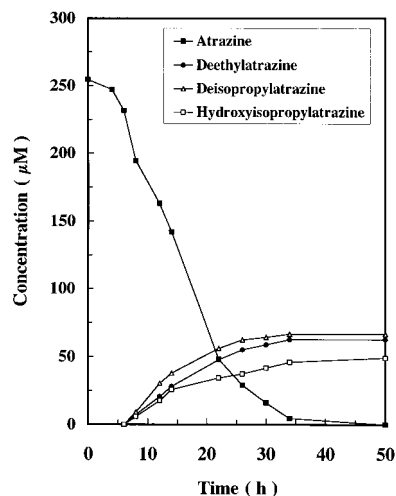
FIG. 1. Degradation of atrazine and accumulation of metabolites by Rhodococcus sp. strain NI86/21 cells growing in BSM with fructose. The cell density (OD 600 ) increased from 0.19 to 1.20 after 50 h.
