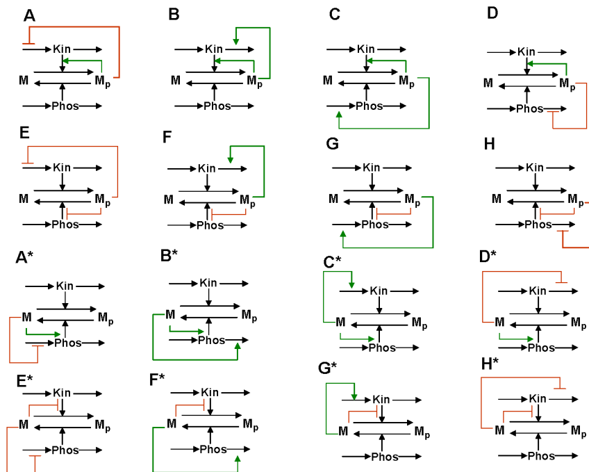
FIG. 2. Feedback designs that can turn a universal signalling cycle into a bistable switch and relaxation oscillator. Simple cycle can turn bistable in four distinct ways; either M_p or M stimulates its own production (positive feedback) by product activation or substrate inhibition of the kinase or phosphatase reactions. Each of the four rows of feedback designs correspond to a different bistable switch, provided that the kinase and phosphatase abundances are assumed constant and only single feedback (within the M cycle) is present. Sixteen relaxation oscillation designs are generated by extra negative feedback brought about by negative or positive regulation of the synthesis or degradation rates of the kinase protein or phosphatase protein by M_p or M . Designs A*-H* are mirror images of designs A-H . Although synthesis and degradation reactions are shown for both the kinase and phosphatase proteins, the protein concentration that is not controlled by feedback from the M cycle is considered constant, resulting in only two differential equations for each diagram. All feedback regulations are described by simple Michaelis-Menten type expressions (BOX 2 and Supplementary Table S3). The remaining sixteen relaxation oscillation designs are shown in Supplementary FIG.S1 and can require some degree of cooperativity within feedback loops.
