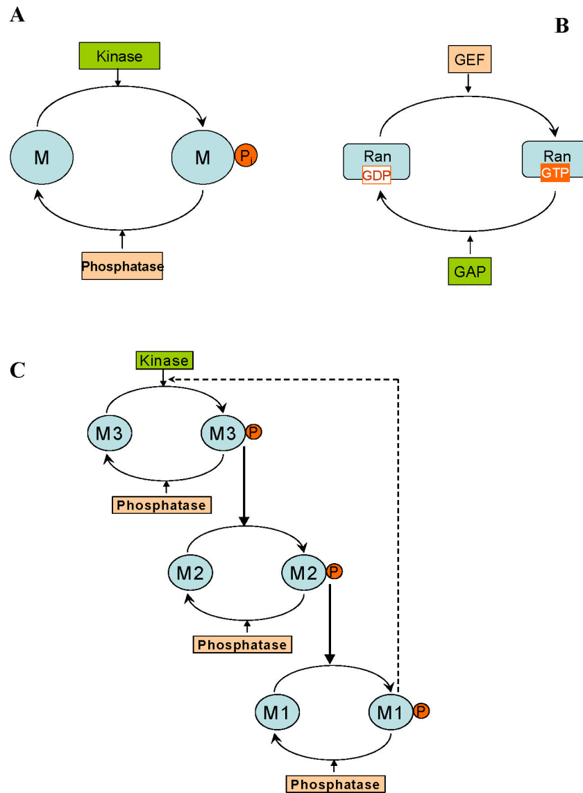
FIG. 1. Universal motifs of cellular signalling networks. A. One-site phosphorylation cycle. The protein M is phosphorylated by a kinase to yield the phosphorylated form M_p , which is dephosphorylated by an opposing phosphatase. B. A cycle of a small GTPase (Ran). A guanine nucleotide exchange factor (GEF) catalyzes the transformation of an inactive guanosine diphosphate (GDP)-bound form (Ran-GDP) into an active guanosine triphosphate (GTP)-bound form (Ran-GTP). A GTPase-activating protein (GAP) is the opposing enzyme that catalyzes the reverse transformation. C. A cascade of cycles. Negative feedback provides robustness to noise, increasing resistance to disturbances inside the feedback loop, but brings about oscillations if it is too strong and the cascade is ultrasensitive 12,20 . Positive feedback greatly increases the sensitivity of the target to the signal and may also lead to bistability and relaxation oscillations 12,18,46,72 .
