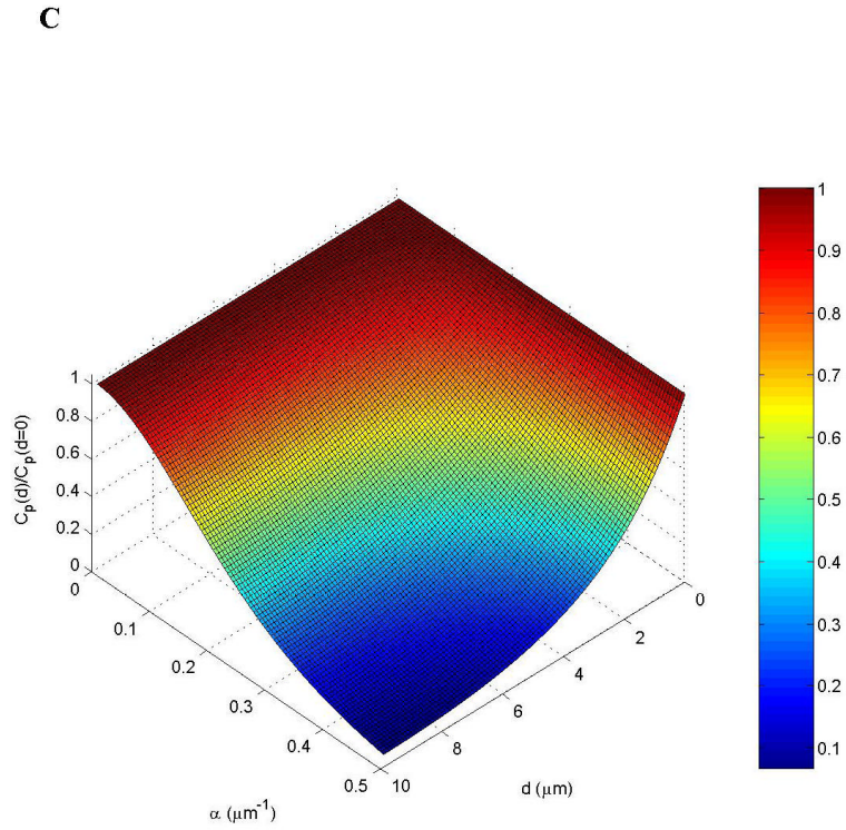
FIG. 3. Spatial segregation of two opposing enzymes in a protein-modification cycle generates intracellular gradients. Kinases localize to (A) supra-molecular structures (sphere) or (B) the cell membrane, whereas phosphatases are homogeneously distributed in the cytoplasm. The concentration gradients are shown by colour intensity. C. Stationary phosphorylation levels c_p decline with the distance d from the cell membrane toward the centre [Brown, 1999 #61 (see panel B ). The steepness of the gradient (reciprocal of the characteristic length) is determined by the parameter \alpha (\alpha^2 = k_p/D is the ratio of the phosphatase activity k_p and the protein diffusivity D , BOX 3).
