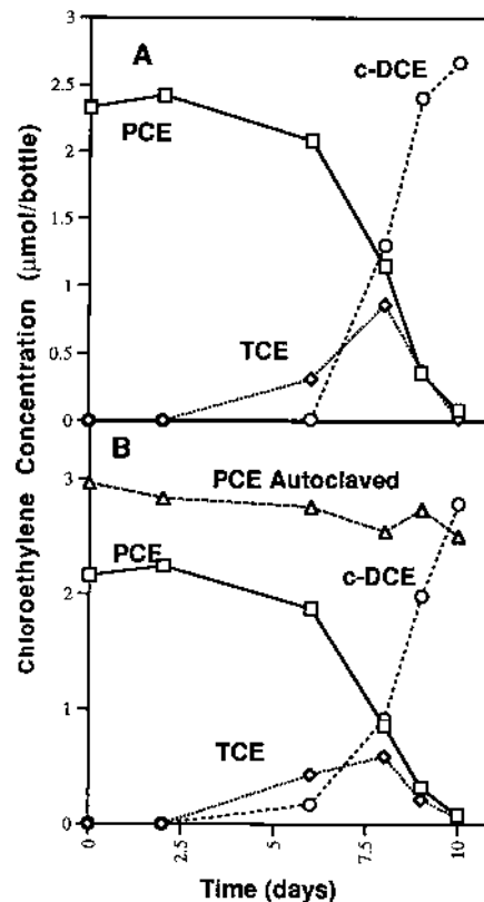
FIG. 1. Plot of the time course of the depletion of PCE and the accumulation of trichloroethylene (TCE) and cis -dichloroethylene (c-DCE) in enrichment cultures incubated with 0.25% agar (A) or 5 mM acetate (B) as the electron donor. Enrichment cultures were incubated in 40-ml serum bottles with 20 ml of a mineral medium.
