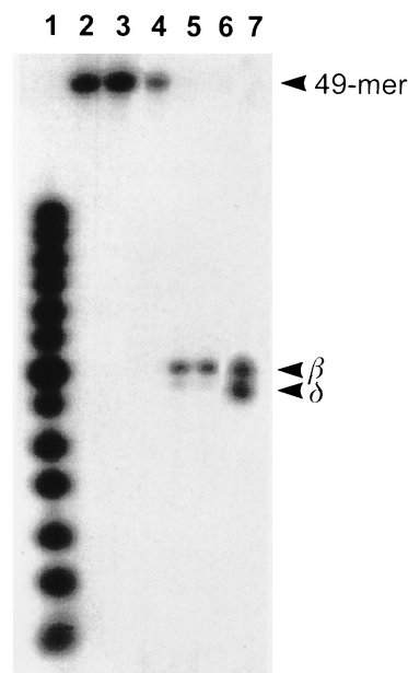
FIG. 3. Pyrimidine dimer-specific nicking activity isolated from PBCV-1-infected chlorella cells. Lanes: 1, oligonucleotide size markers (8 to 32 bases); 2 and 3, 5'-end-labelled duplex 49-mer oligonucleotide containing a centrally located cyclobutane pyrimidine dimer incubated alone (lane 2) or with extracts from purified virions (lane 3); 4, uninfected chlorella; 5, chlorella cells at 90 min after PBCV-1 infection; 6, chlorella cells 180 min after PBCV-1 infection; 7, T4 endonuclease V enzyme.
