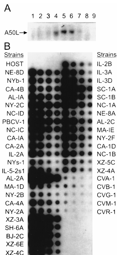
FIG. 4. (A) Northern blot analysis of RNAs isolated from uninfected and from PBCV-1-infected chlorella cells at 15, 30, 45, 60, 90, 120, 240, and 360 min after infection (lanes 1 to 9, respectively). The blot was hybridized with the A50L gene. (B) Hybridization of the PBCV-1 A50L gene to DNA isolated from the host Chlorella strain NC64A and from 37 chlorella viruses that infect Chlorella strain NC64A and 5 viruses (CVA-1, CVB-1, CVG-1, CVM-1, and CVR-1) that infect Chlorella strain Pbi. The blots contain 1, 0.5, 0.25, and 0.12 \mu g of DNA, left to right, respectively. Note that the A50L gene did not hybridize to the host chlorella DNA even after prolonged exposure.
