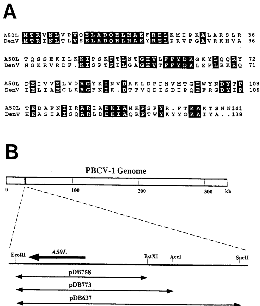
FIG. 1. (A) Sequence alignment of PBCV-1 ORF A50L with bacteriophage T4 endonuclease V (T4endoV) was performed. (B) The PBCV-1 ORF A50L was subcloned from cosmid cYL5 by using DNA restriction endonuclease SacII , AccI , or BstXI to cleave 1,168 bp (pDB637), 667 bp (pDB773), or 475 bp (pDB758), respectively, upstream of the translational start codon of the gene and EcoRI to cleave 105 bp after the translational stop codon of the gene. Each fragment was inserted into the polylinker region of pBluescript KS(+).
