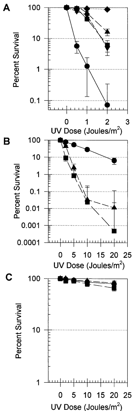
FIG. 2. (A) UV sensitivity of E. coli AB2480 ( uvrA recA ) with and without plasmids containing the PBCV-1 A50L gene. E. coli AB2480 contained pBlue-script KS(+), pDB637 (squares), pDB773 (inverted triangles), or pDB758 (triangles). E. coli AB1157 ( uvrA + recA + ) served as the control (diamonds). Means and standard errors are illustrated. (B and C) UV inactivation of PBCV-1 virus and two deletion mutants lacking the A50L gene under dark repair (B) and light repair conditions (C). PBCV-1 wild type (circles) and deletion mutants P1050 (squares) and P1210 (triangles) are shown. Means and standard errors are illustrated.
