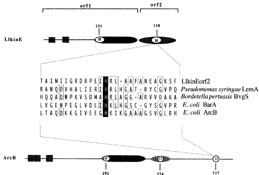
FIG. 5. Alignment of a short region of similarity between proteins belonging to the unorthodox kinase family (9) and the corresponding region of LkinEorf2. The central histidine, which is the only completely conserved residue, is indicated by a solid box. Amino acids are boxed if at least three of the depicted protein sequences contain an identical residue at a particular position. The relative positions of the compared sequences and the organization of the corresponding genes are shown in the schematic structures of the representatives of E. coli ArcB and L. lactis LkinEorf2. The numbers refer to the positions of the conserved histidine and aspartate residues in each of these proteins.
