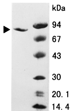
FIG. 2. Sodium dodecyl sulfate-PAGE of purified KOD DNA polymerase. The gel was stained with Coomassie brilliant blue R-250.
