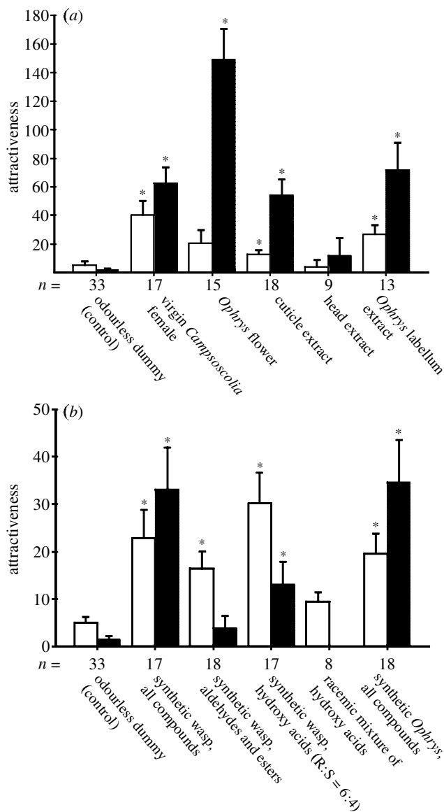
Figure 1. Attractiveness (mean \pm s.e.m.) of (a) intact freeze-killed virgin females, Ophrys flowers, various odour samples obtained from virgin females and Ophrys flowers, and (b) synthetic mixtures to C. ciliata males. Odourless dummies (Soxhlet-extracted dried C. ciliata females) impregnated with odour samples were offered to the males. Assays were carried out for 3 min, and two different male reactions were recorded: pouncing on the dummy (open bars) and attempts to copulate with the dummy (filled bars). In each assay individual reactions of males were divided by the number of patrolling males crossing a 1 m long wire and multiplied by 100. Columns marked with an asterisk differ significantly from the odourless dummy (Mann–Whitney U -test, p < 0.005 ).
