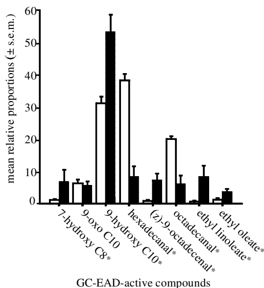
Figure 3. Comparison of relative proportions (mean \pm s.e.m.) of electrophysiologically active compounds in cuticle extracts of virgin C. ciliata females (filled bars) ( n = 4 ) and labellum extracts of O. speculum flowers (open bars) ( n = 16 ). Asterisks indicate significant difference, Mann-Whitney U -test, p < 0.01 . Three to five individuals were pooled for each of the four C. ciliata samples because of the small amounts of the target compounds. The total number of females investigated was 15. For statistical analyses the values equivalent to single females were used.
