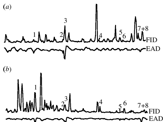
Figure 2. Simultaneous flame ionization/detection (FID) and electroantennographic-detection (EAD) analyses performed with (a) a cuticle extract of a C. ciliata female and (b) an O. speculum labellum extract. Numbered peaks correspond to compounds that elicit electroantennographic responses: 1, 7-hydroxyoctanoic acid; 2, 9-oxodecanoic acid; 3, 9-hydroxydecanoic acid; 4, hexadecanal; 5, (z)-9-octadecenal; 6, octadecanal; 7, ethyl linoleate; 8, ethyl oleate. In order to detect all 'physiologically active' compounds and to discriminate electrophysiological responses from noise we performed five to 10 GC-EAD runs for each type of sample.
