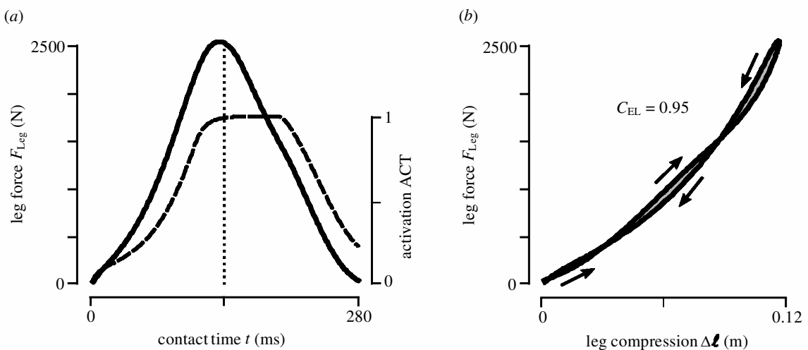
Figure 5. Example of the hopping pattern using F+. (a) The leg force (solid line) and muscle activation (dashed line), and (b) the leg force–length curve ( \Delta l = \ell_{F-y} ) of the steady-state hopping pattern used for the sensitivity analysis are shown ( STIM_0 = 0.145 , G = 1.84/F_{max} ). The shaded area enclosed by the force–length curve depicts the area A used for the calculation of the elasticity coefficient C_{EL} (equation (2.10)).
