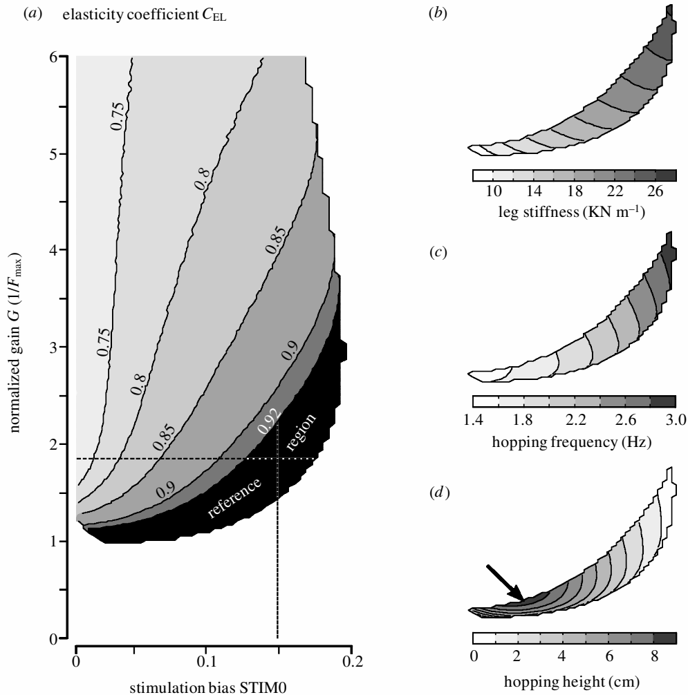
Figure 4. Elastic leg behaviour. The model behaviour using F+ is mapped throughout the feedback parameter space ( STIM_0 , G ). (a) The elasticity coefficient C_{EL} for stable hopping patterns (shaded area) is shown. The intersection of the dashed lines refers to the parameters used for sensitivity analysis ( STIM_0 = 0.145 , G = 1.84/F_{max} ; see figure 5). (b–d) In the reference region the elasticity coefficient exceeds the reference value of C_{EL} = 0.92 (see (a)). Here, the corresponding (b) leg stiffness, (c) hopping frequency and (d) hopping height are shown. The arrow indicates the maximum hopping height within the reference region ( STIM_0 = 0.065 , G = 1.32/F_{max} ).
