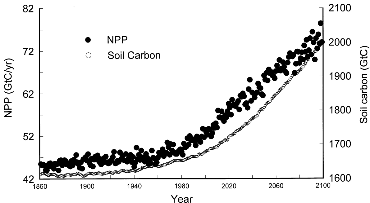
Figure 7. Predicted trends in vegetation net primary productivity and soil carbon after feedback of vegetation on atmospheric \text{CO}_2 partial pressure.
