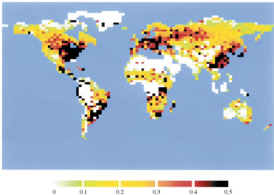
Figure 11. Difference map of global net primary productivities (NPPs) in the control run for the 2090s less the NPPs for vegetation feedbacks on atmospheric CO 2 and temperature.
