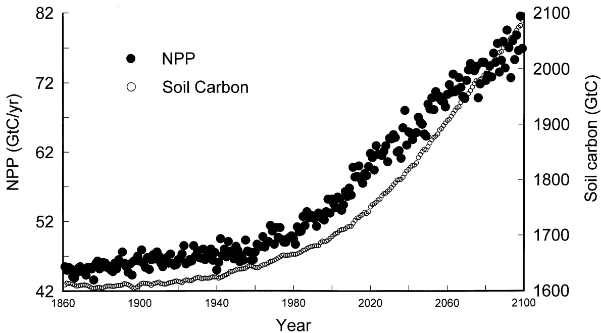
Figure 3. Predicted trends in vegetation net primary productivity and soil carbon, using the climate and \text{CO}_2 data from Mitchell et al. (1995) as input drivers of a vegetation model (Woodward et al. 1995). Control: no vegetation feedback.
