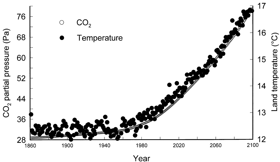
Figure 2. Trends in annual land surface temperature and atmospheric \text{CO}_2 partial pressure, as predicted in Mitchell et al. 's (1995) transient climate projection. Control: no vegetation feedback.
