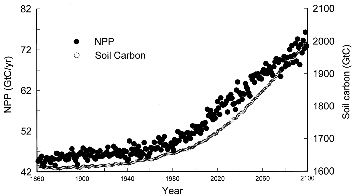
Figure 10. Predicted trends in vegetation net primary productivity and soil carbon after feedback of vegetation on atmospheric \text{CO}_2 partial pressure and temperature.
