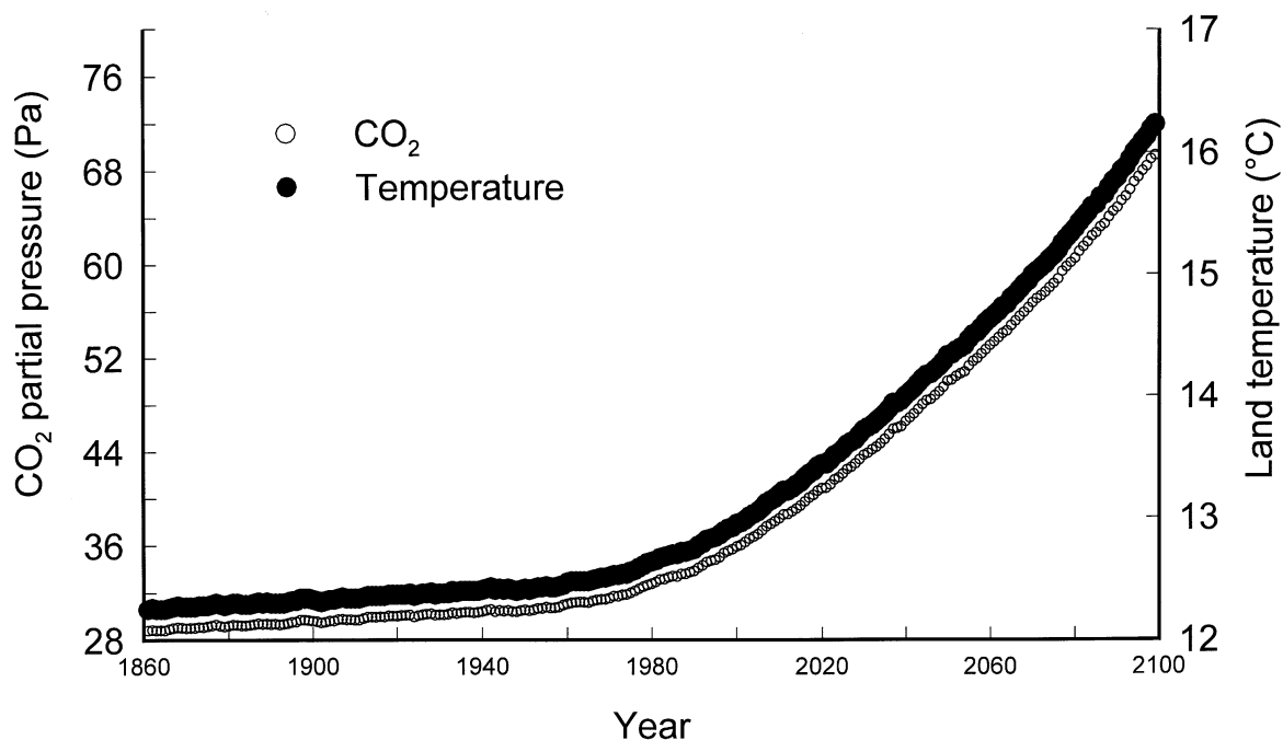
Figure 9. Trends in annual land surface temperature and atmospheric \text{CO}_2 partial pressure after feedback of vegetation on atmospheric \text{CO}_2 partial pressure and temperature. The changes in temperature are calculated from the regression equation of land surface temperature on \text{CO}_2 partial pressure (from figure 2): T = (9.45 \times 0.0973)C , where T is temperature ( ^{\circ}\text{C} ) and C is \text{CO}_2 partial pressure (Pa).
