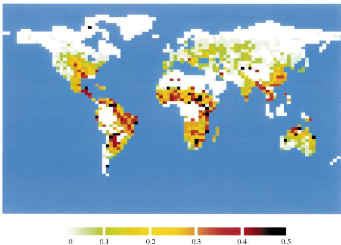
Figure 8. Difference map of global net primary productivities (NPPs) in the control run for the 2090s less the NPPs for vegetation feedbacks on atmospheric \text{CO}_2 .
