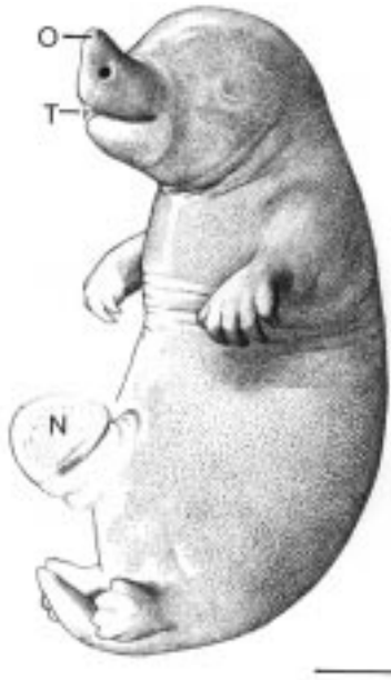
Figure 7. Drawing of a newly hatched O. anatinus , (specimen WW), from the Hill collection. Eyelids now cover the eyes, digits have appeared on the hindfeet, there is a prominent yolk navel (N), oscaruncle (O), and egg tooth (T). Scale bar, 2 mm.
