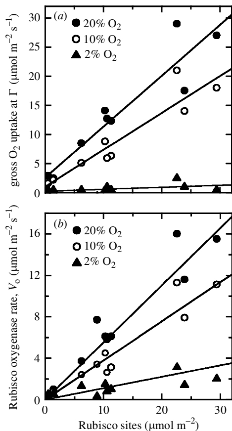
Figure 2. (a) Gross \text{O}_2 uptake rates and (b) rubisco oxygenase rates, V_0 at the \text{CO}_2 compensation point, \Gamma . The data in (b) were calculated from (a), as a function of rubisco site concentrations in wild-type and anti-SSu tobacco plants. Measurements were made at 20%, 10% and 2% \text{O}_2 and 25 °C. The calculation of V_0 was as previously described (Ruuska et al. 2000). The lines are the theoretical oxygenase or \text{O}_2 uptake rates predicted from the equation for oxygenase rates (for a review, see Ruuska et al. 2000).
