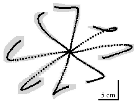
Figure 9. After-effects of adaptation. Average and standard deviations of hand trajectories executed at the end of training in the field when the field was unexpectedly removed on random trials. Compare these trajectories with the initial-exposure movements of figure 7 d . (From Shadmehr & Mussa-Ivaldi 1994.)
